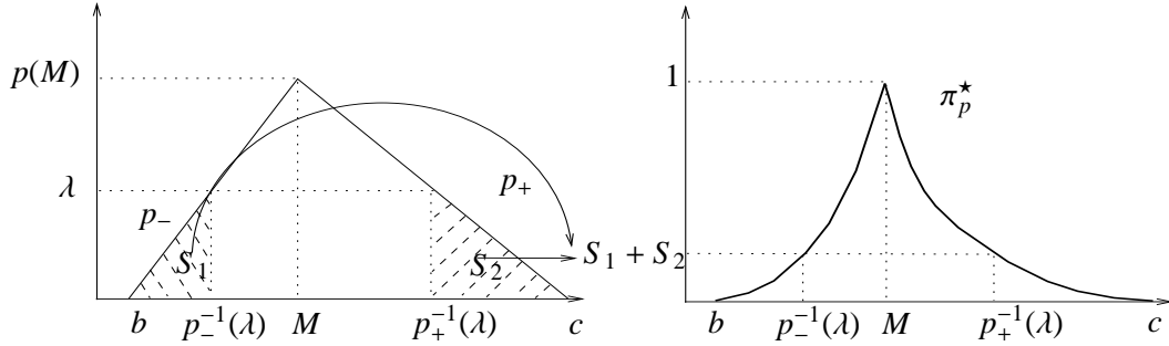
Fig. B.1. Triangular probability density p on the left and the shape of its \pi_p^\star optimal transformation on the right.
