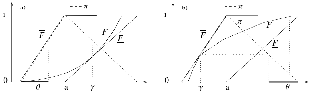
Fig. 1. Probabilities in \mathcal{P}(\underline{F} < \bar{F}) but not in \mathcal{P}(\pi) .
