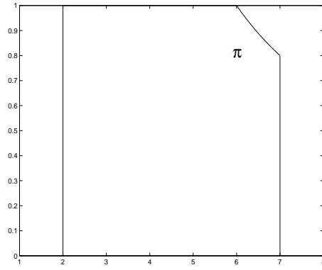
Fig. 4. Possibility distribution \pi containing the probability box [\underline{F}, \overline{F}] .
