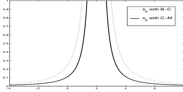
Fig. 6. Optimal possibility distribution \pi_p knowing \mu = 2 and \sigma = 1 and using Bien-aymé-Chebychev and Camp-Meidel inequality.
