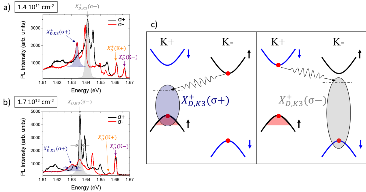
Figure 4. Photoluminescence spectra measured at B=9 T for (a) low ( 1.4 \times 10^{11} \text{ cm}^{-2} ) and (b) large ( \sim 1.7 \times 10^{12} \text{ cm}^{-2} ) hole doping densities; (c) schematics of the optical transition associated to the K_3 phonon replica of the positive dark trion, X_{D,K3}^+ .
