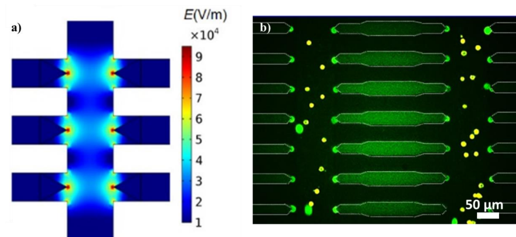
Figure 8 a) 2D simulation of the electric field distribution across a single microchannel flanked by 6 BE tips. b) Fluorescent image showing the capture of single MDA-MB-231 cells (green) in the presence of Jurkat cells (yellow) by applying an AC field using a BE array. Reprinted from reference (116) with permission from the American Chemical Society .
