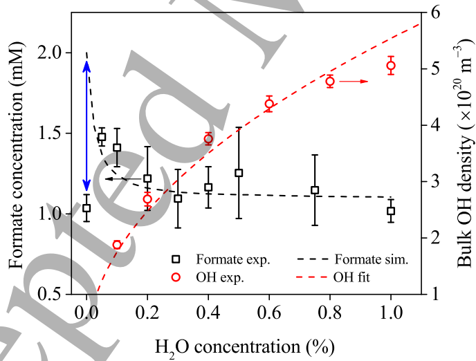
Figure 11. Average formate concentration in plasma-treated droplets as a function of water concentration in He/ \text{H}_2\text{O} plasma, compared with the 1D diffusion-reaction modeling result. The discharge was operated at a total gas flow rate of 1.5 slm ( t_{\text{res}} = 8 \text{ ms} ), and fixed power of 14.3 \pm 0.5 \text{ W} for He/ \text{H}_2\text{O} plasmas and 13.6 \pm 1.3 for pure He plasma. The corresponding \cdot\text{OH} densities are taken from [53] and follow the following relation: n_{\text{OH}}[\text{m}^{-3}] = 5.54 \times 10^{20} \sqrt{n_{\text{H}_2\text{O}}[\%]} .
