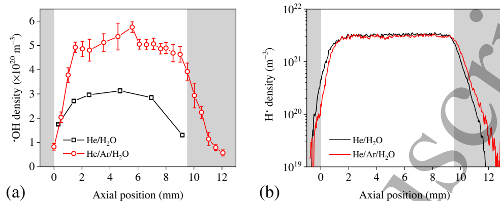
Figure 8. Absolute number densities of (a) \cdot\text{OH} radicals, and (b) \text{H}\cdot radicals measured as a function of the axial position in the bulk of He + 0.2% \text{H}_2\text{O} and He + 17% Ar + 0.2% \text{H}_2\text{O} plasmas at a gas flow rate of 1.0 slm. The data for \cdot\text{OH} density in He + 0.2% \text{H}_2\text{O} plasma in (a) is taken from [10]. The white region represents the location of the electrodes in the axial direction.
