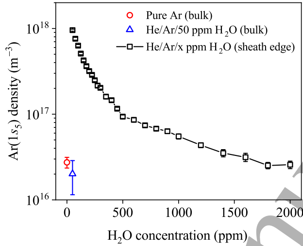
Figure 7. Time-averaged absolute densities of Ar( 1s_5 ) metastable atoms in He + 17% Ar + x ppm H 2 O plasma as a function of H 2 O concentration at a total gas flow rate of 5 slm. The power varied from 14.3 W to 13.4 W corresponding to 50 ppm and 2000 ppm H 2 O, respectively. The measurements were taken at the position of the maximum density of Ar( 1s_5 ) atoms near the sheath edge. The densities of Ar( 1s_5 ) metastable atoms in the bulk of the discharge in pure Ar and He + 17% Ar + 50 ppm H 2 O plasmas are also shown.
