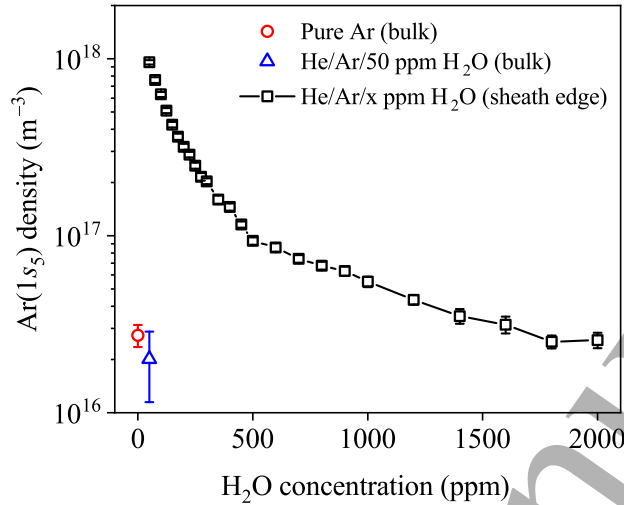
Figure 7. Time-averaged absolute densities of \text{Ar}(1s_5) metastable atoms in \text{He} + 17\% \text{Ar} + x \text{ppm H}_2\text{O} plasma as a function of \text{H}_2\text{O} concentration at a total gas flow rate of 5 slm. The power varied from 14.3 W to 13.4 W corresponding to 50 ppm and 2000 ppm \text{H}_2\text{O} , respectively. The measurements were taken at the position of the maximum density of \text{Ar}(1s_5) atoms near the sheath edge. The densities of \text{Ar}(1s_5) metastable atoms in the bulk of the discharge in pure Ar and \text{He} + 17\% \text{Ar} + 50 \text{ppm H}_2\text{O} plasmas are also shown.
