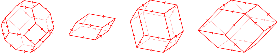
FIGURE 5. Linear orientations of the graphs of the graphical zonotopes corresponding to the acyclic reorientation posets of Figure 1. The first is the classical permutohedron (which has been rescaled to fit the size of the others). The perspective is chosen so that the minimal reorientation appears at the bottom of the picture.
