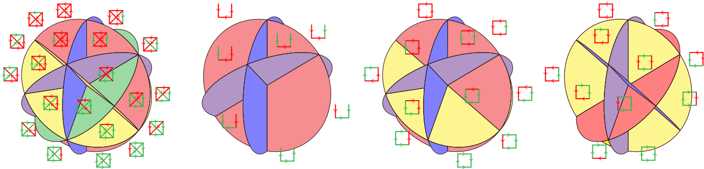
FIGURE 4. The graphical arrangements corresponding to the acyclic reorientation posets of Figure 1. The first is the classical braid arrangement. The regions are labeled by the corresponding acyclic reorientations. The hyperplanes are colored according to the corresponding arc. The perspective is chosen so that the minimal reorientation appears at the bottom of the picture.
