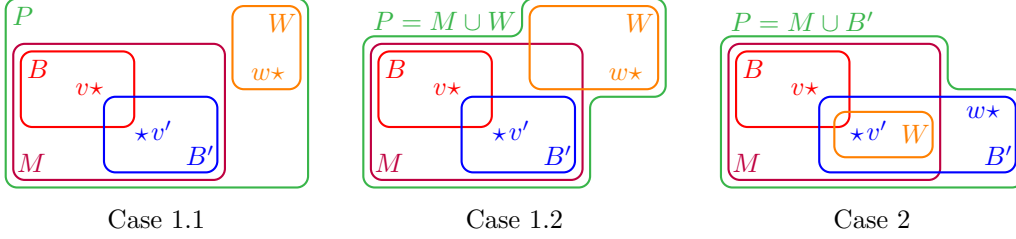
FIGURE 6. Illustrations for the case analysis of the proof of Theorem 3.23.
