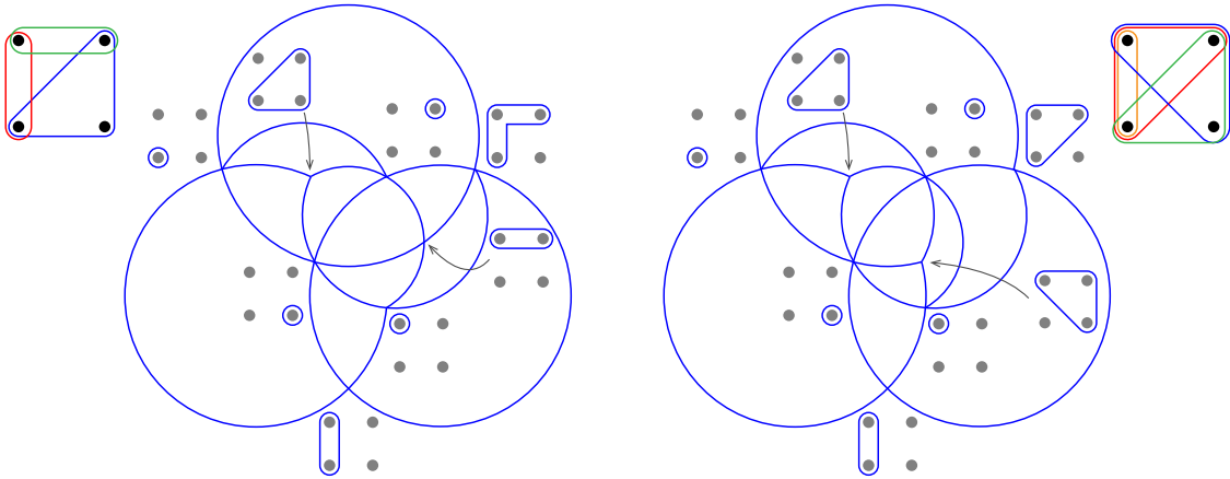
FIGURE 5. Two nested fans. As the fans are 3-dimensional, we intersect them with the sphere and stereographically project them from the direction (-1, -1, -1) .
