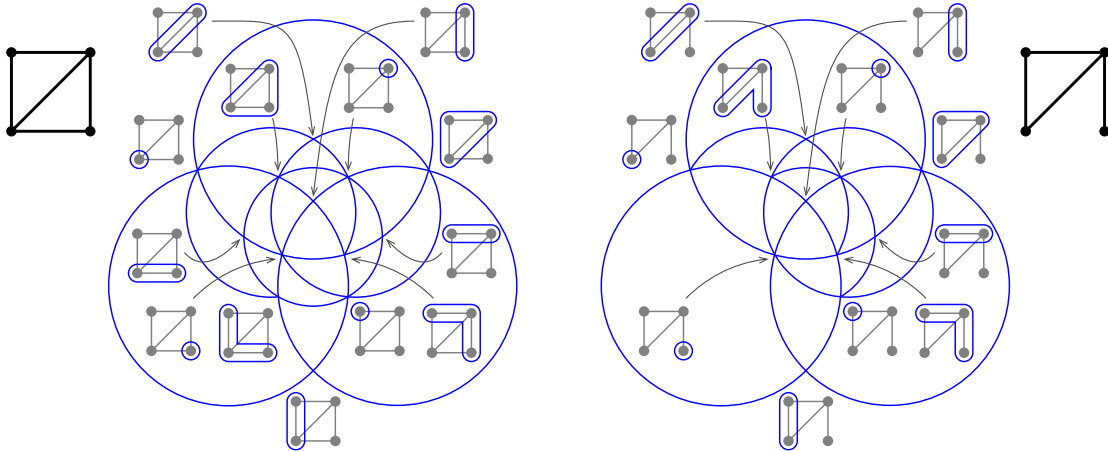
FIGURE 3. Two graphical nested fans. As the fans are 3-dimensional, we intersect them with the sphere and stereographically project them from the direction (-1, -1, -1) .
