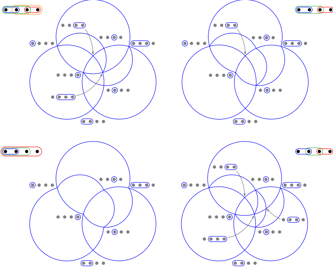
FIGURE 7. Four interval nested fans. The bottom left one is the Pitman-Stanley fan, the bottom right one is the Sylvester fan. As the fans are 3-dimensional, we intersect them with the sphere and stereographically project them from the direction (-1, -1, -1) .
