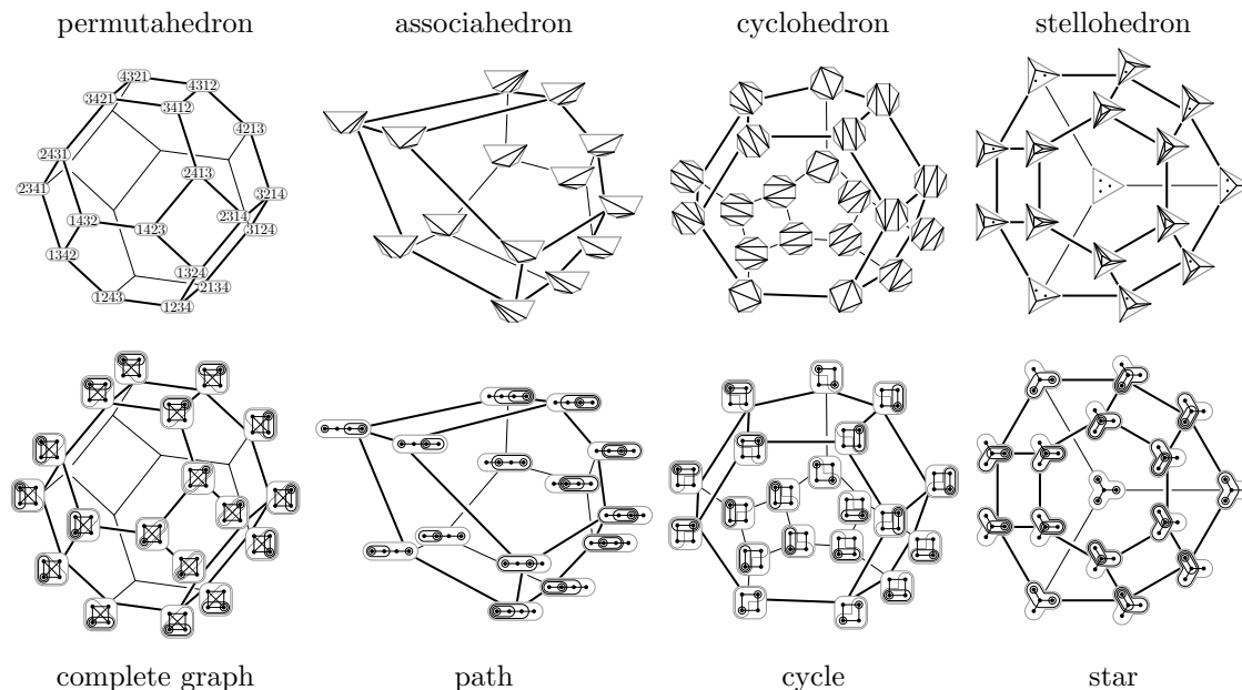
FIGURE 1. Some classical families of polytopes as graph associahedra. Illustration from [MP17].
