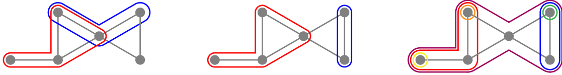
FIGURE 2. Some incompatible tubes (left and middle), and a maximal tubing (right).
