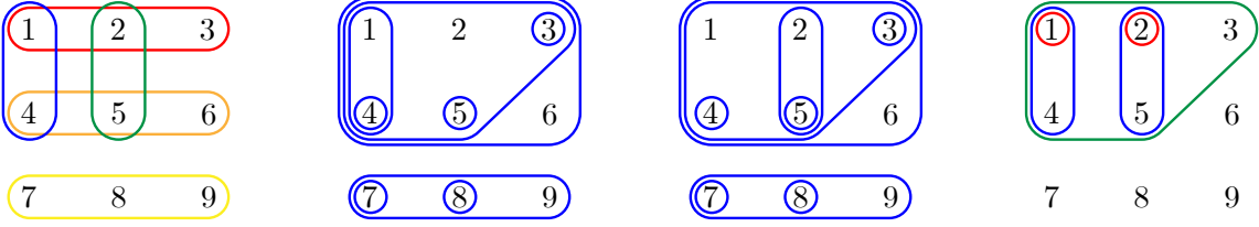
FIGURE 4. The elementary blocks of a building set \mathcal{B}_0 (left), two adjacent maximal \mathcal{B}_0 -nested sets (middle), and the corresponding frame (right).
