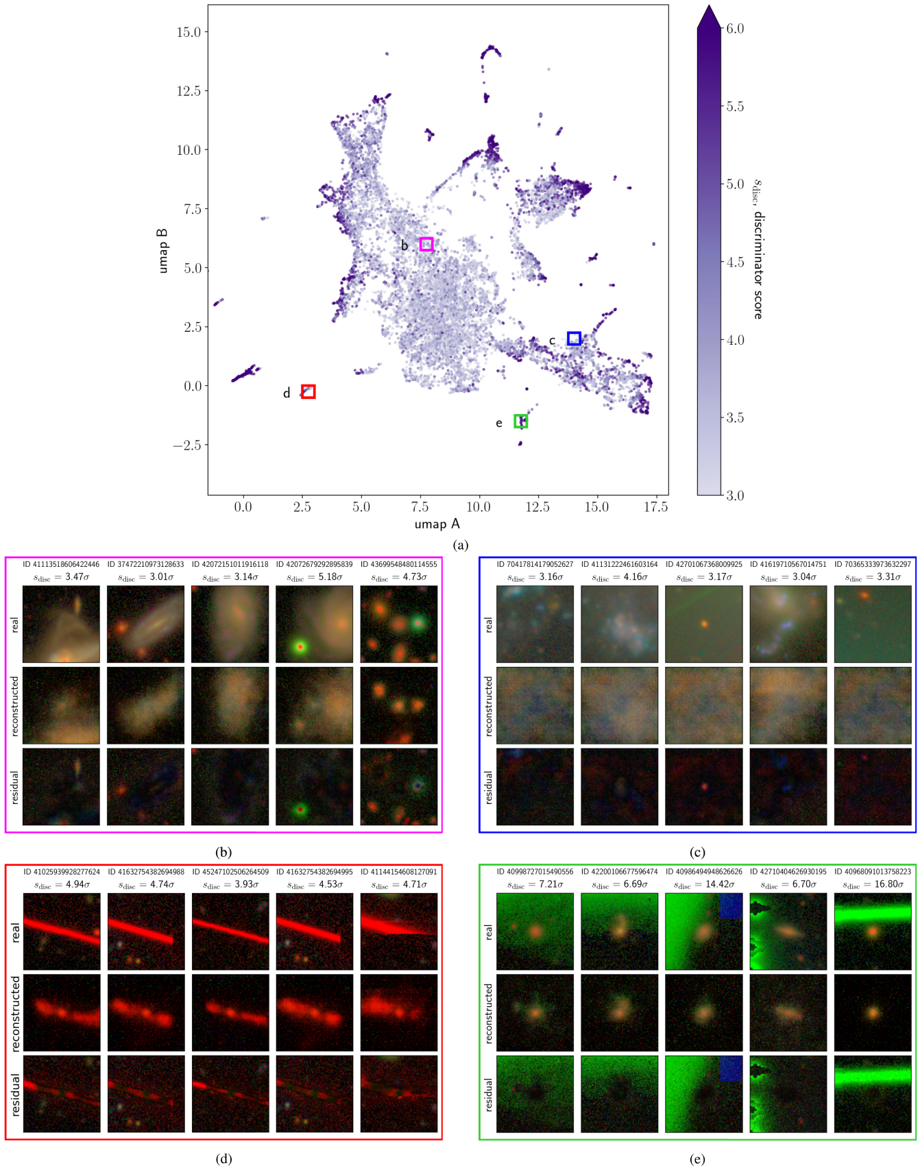
Figure 9. A visualization of our anomaly characterization method with our WGAN-based anomaly scores and autoencoded residual images. Panel (a) shows a UMAP embedding of all anomalies with s_{disc} > 3\sigma above the mean, colour-coded by anomaly score. Panels (b)–(e) show a random selection of galaxies in each of UMAP regions enclosed by the box of the corresponding colour in panel (a). It is clear that different regions of the UMAP correspond to different types of anomalies, including both interesting objects [as in (b) and (c)] and corrupted images [as in (d) and (e)].
