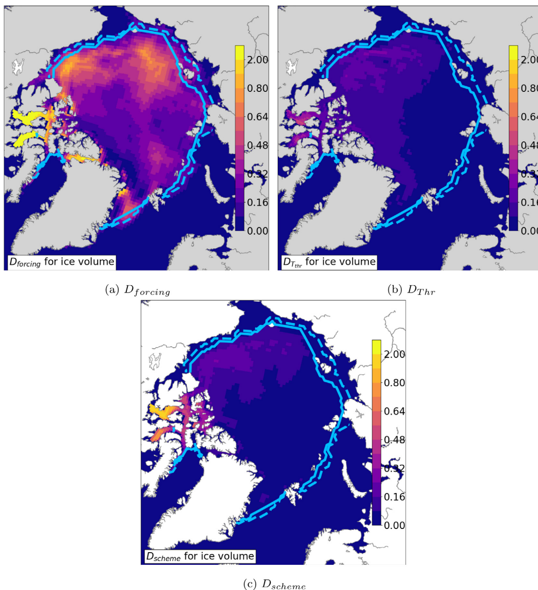
Fig. 11. Mean absolute differences of sea ice volume attributed to the forcing (11(a)), T_{thr} (11(b)) and melt pond scheme (11(c)) in September over 1980–2011, in m^3 per grid cell area. The light blue continuous (dashed) line indicates the 15% ice concentration contour of the simulation with the smallest (largest) ice extent.
