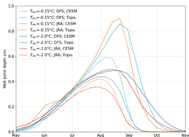
Fig. 8. Mean seasonal cycles of the effective meltwater depth in the melt ponds over 2000–2011 for the different simulations carried out with NEMO-LIM.
