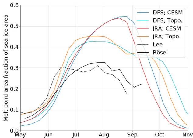
Fig. 7. As Fig. 1 but for the group of simulations with T_{thr} set equal to -2.00\text{ }^{\circ}\text{C} . The mean seasonal cycles derived from the datasets of Rösel et al. (2012) and Lee et al. (2020) are drawn in black.
