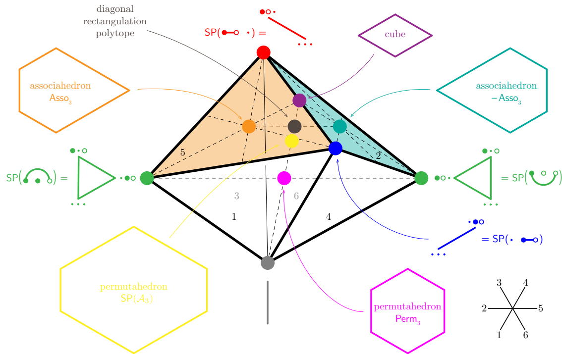
Figure 7: The type polytope of the permutahedron \text{Perm}_3 .
