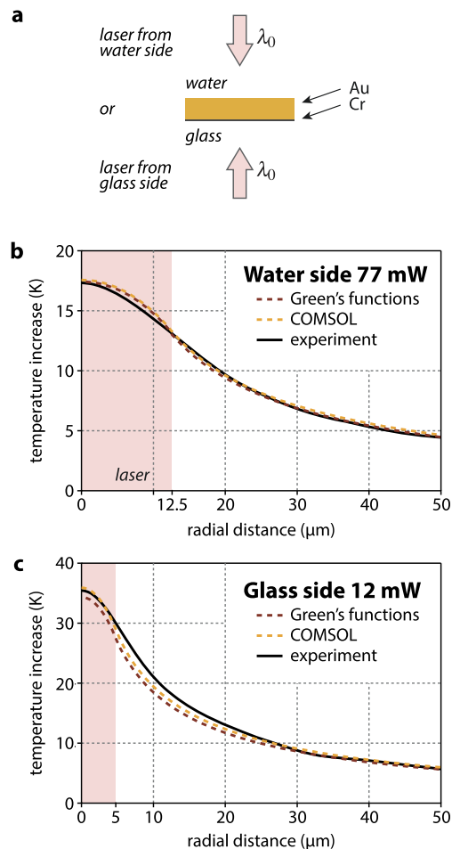
FIG. 5. Comparison between numerical simulation (COMSOL and Green's functions) and experimental measurements of the temperature profile of a gold film under illumination by a uniform laser beam at \lambda = 790 nm. (a) Schematic of the system, consisting of a 100 nm gold layer, supported on a 5 nm thick Cr adhesion layer, illuminated either from the top or from below. (b) Temperature profiles for the case of top illumination, with a beam diameter of 25 \mu\text{m} . In that case, the Cr layer has no effect on the light absorption. The models did not consider it. Experiments were conducted with a 40\times water immersion objective. (c) Temperature profiles for the case of bottom illumination, with a beam diameter of 9.5 \mu\text{m} . The Cr layer thickness was used as a free parameter, set to 6.05 nm, a value fully consistent with the estimation. Experiments were conducted with a 100\times oil-immersion objective.
