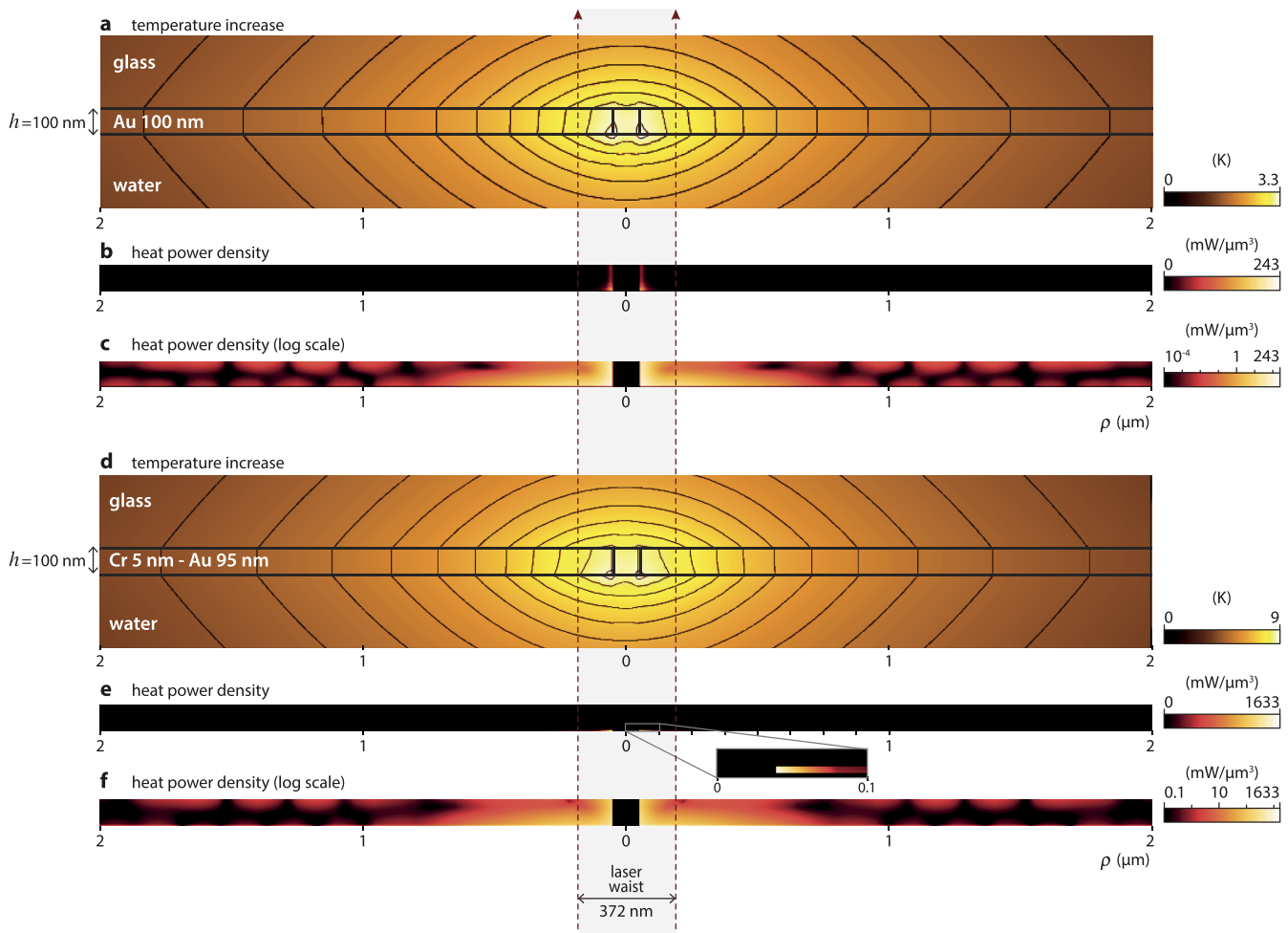
FIG. 10. Consol simulations of the heat power density and the temperature distributions in a glass/metal/water system pierced with a nanohole and illuminated by a focused laser beam at \lambda_0 = 650 nm. (a) Temperature distribution for a gold layer, 100-nm thick and 100-nm nanohole. (b) Associated heat power density. (c) Same as (b) in log colorscale. (d)–(f) Same as (a)–(c) for a 95-nm thick gold layer adhering on a 5-nm thick Cr layer. In (e), a zoom window highlights the heat generation confined in the thin Cr adhesion layer.
