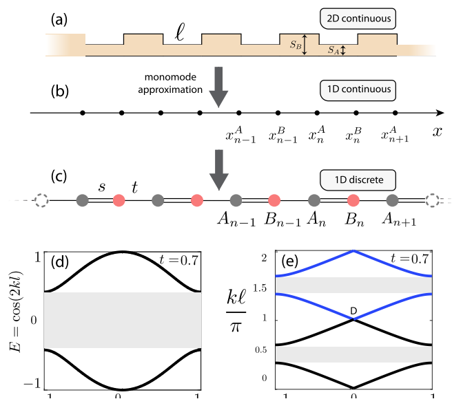
FIG. 1. (a) A sketch of a 2D acoustic waveguide composed of segments of the same length \ell and different cross sections S_A and S_B . (b) Under the monomode approximation the acoustic pressure depends only on the axial coordinate x . On this axis, we can identify the points where the cross sections change. (c) The explicit map onto the SSH discrete model. [(d),(e)] The dispersion relation of the SSH model as given by Eq. (15).
