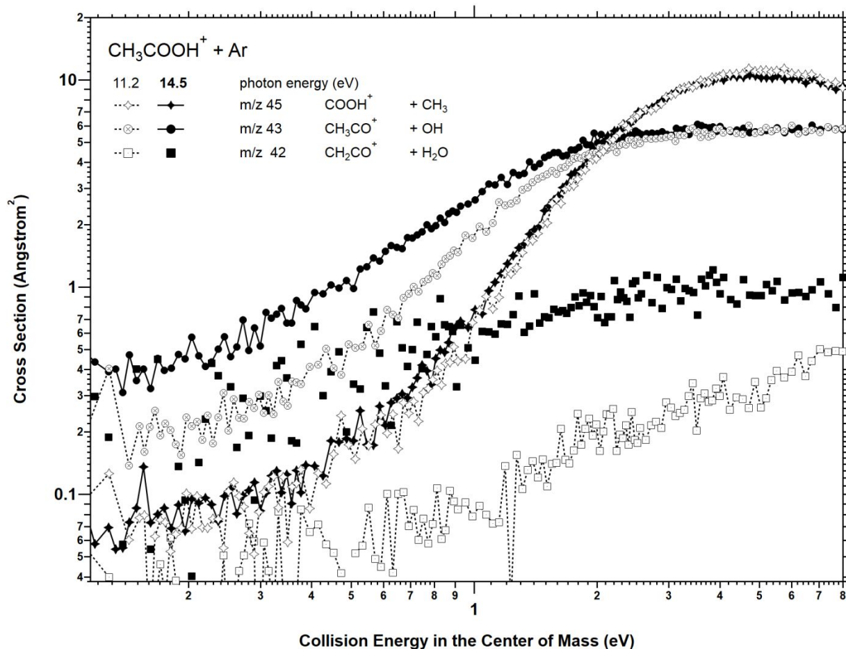
Figure 4: Absolute fragmentation cross sections of CH 3 COOH + colliding with argon as a function of the center of mass collision energy. Results obtained when performing photoionization of acetic acid with 11.2 eV photons are presented with empty symbols, while results at 14.5 eV are presented with filled symbols
