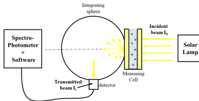
Figure 5. Schematic of the optical bench set up for experimental assessment of the transmittance.
