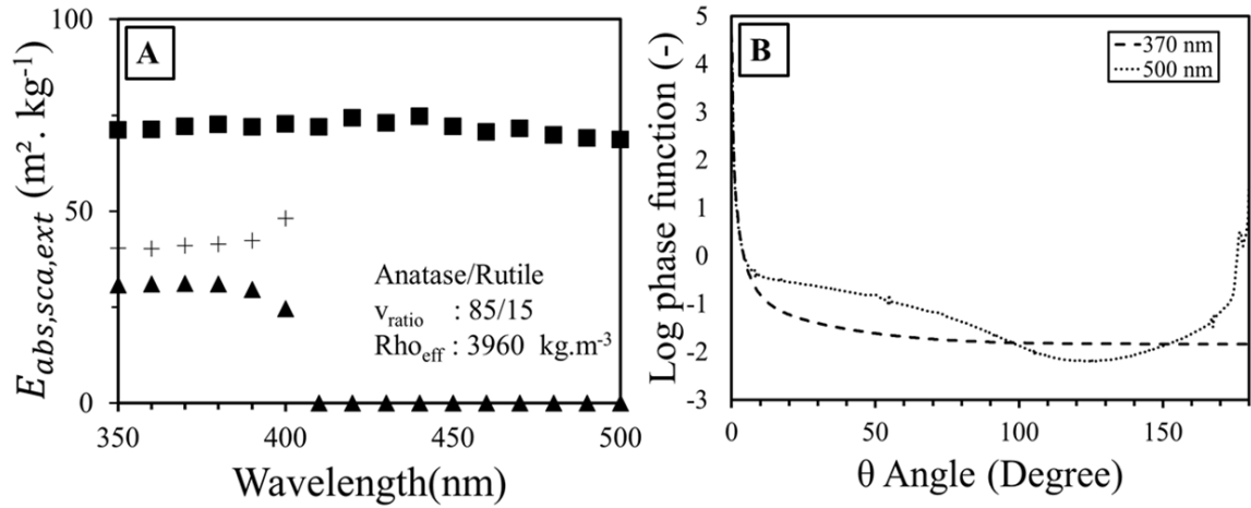
Figure 6. TiO 2 radiative properties assessed by Mie theory: absorption (▲), scattering (+) and extinction (■) specific coefficients from near UV to visible wavelength (A); angle-dependent scattering function in near UV and visible spectral region (B).
