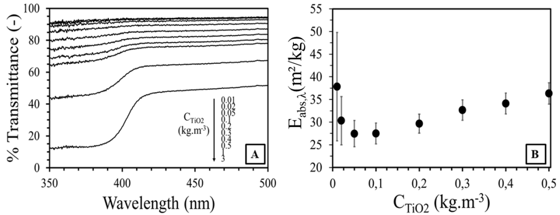
Figure 7. \text{TiO}_2 suspension, experimental transmittance measurement of different concentrations, from near UV to visible wavelength (A). Mean E_{\text{abs},360-390 \text{ nm}} was calculated from experimental transmittance and represented as a function of concentration (B).
