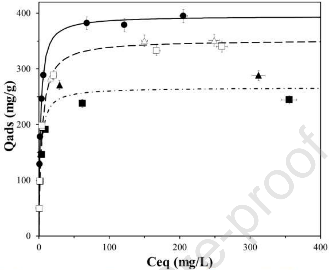
Figure 7. Adsorption isotherms for caffeine onto raw Activated Carbon (●) intermittently milled at different time: 1h-IM-AC (▲); 10h-IM-AC (■). Comparison with Composites Activated Carbon/TiO 2 prepared by mechano-synthesis using the intermittent protocol: 1h-IM-AC/TiO 2 (△); 10h-IM-AC/TiO 2 (□). The continuous and dash lines correspond to the fitted Langmuir model.
