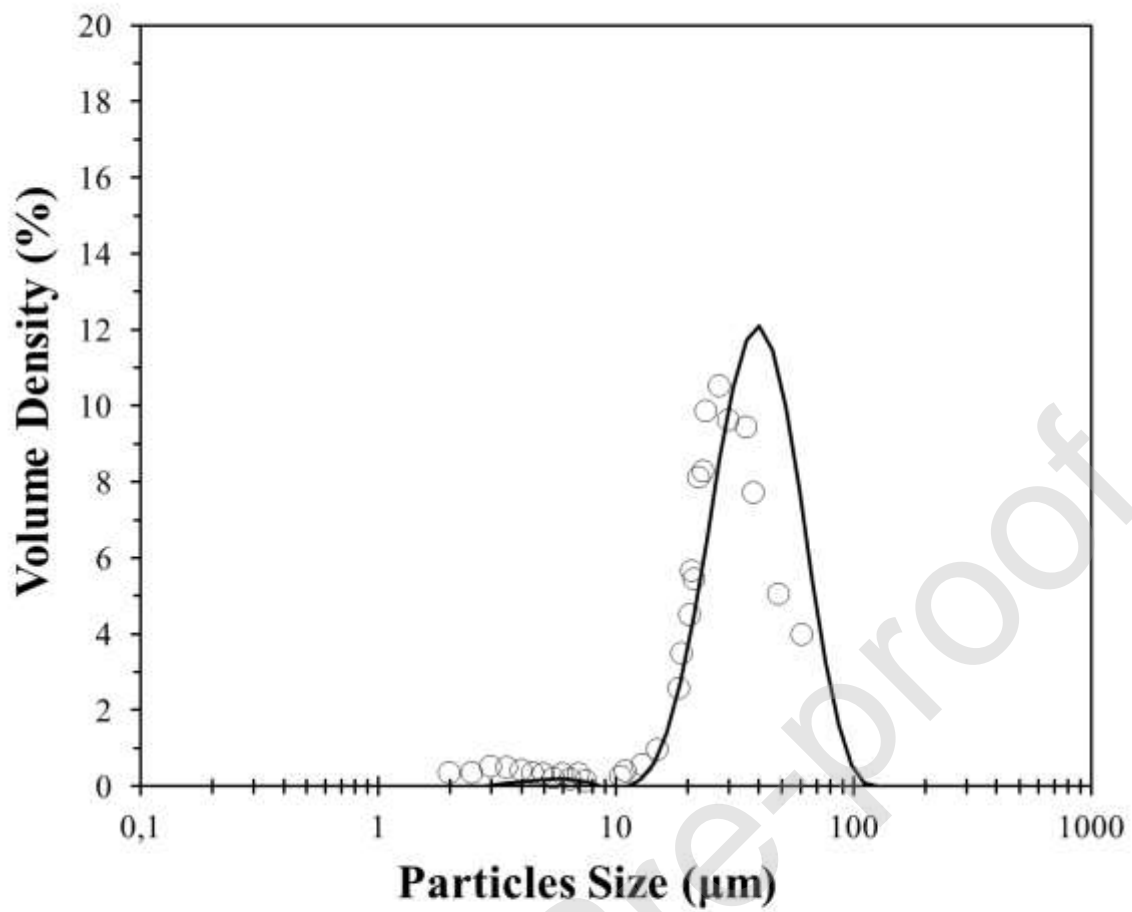
Figure 4. Particles size distribution of Raw TiO 2 . Cross-check between DLS (-) and Image treatment (o) methods.
