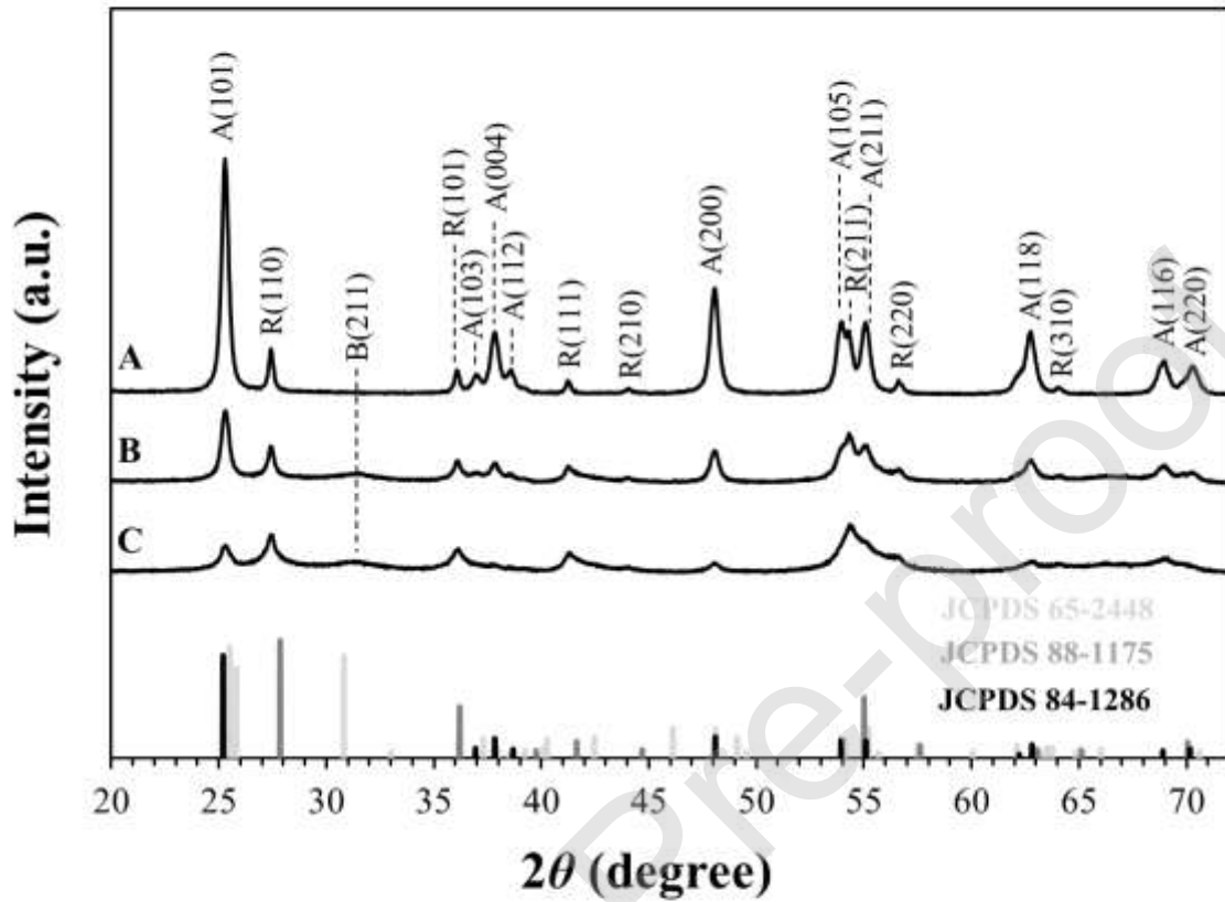
Figure 1. XRD pattern of the raw unmilled TiO 2 (sample a) compared with 10h-IM-TiO 2 (sample b) and 10h-CM-TiO 2 (sample c). Anatase (A), Rutile (R) and Brookite crystal planes are indexed as well as their matching JCPDS data files: respectively JCPDS n° 84-1286; 88-1175; 65-2448.
