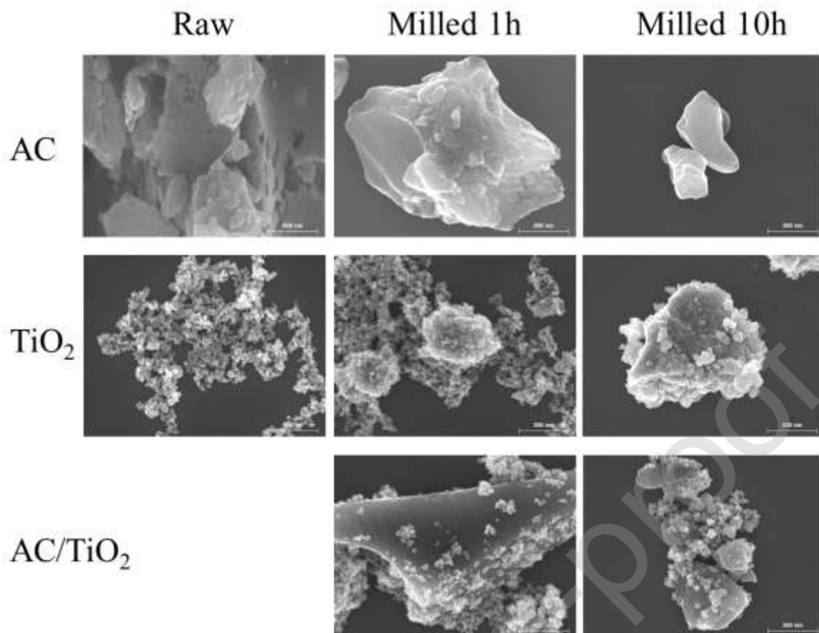
Figure 3. Scanning electron images (SEM-FEG, Hitachi S-4500) of raw and milled samples. Images recorded with a secondary electron detector at 5 kV electron beam for a working distance of 5 mm and a x 50 000 magnification. Left to right: increasing milling time as shown on top. Top to bottom: milled material as shown on the left (AC; TiO 2 ; AC/TiO 2 composites).
