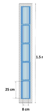
Figure 4: Extraction surface composed of five plasma grids (PG); each grid is drilled with five slits of 25 cm height, 1 cm width.
