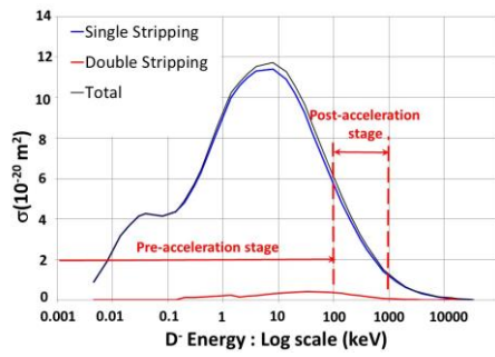
Figure 5: Cross section of D^- stripping (and double stripping) in function of D^- energy.
