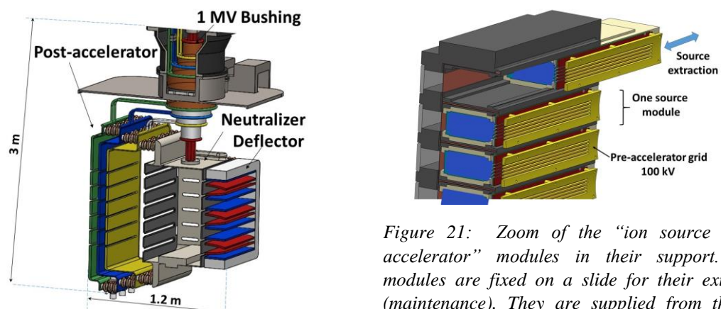
Figure 20: High voltage assembly comprising the bushing, the post-accelerator, the neutralizer and deflector.
