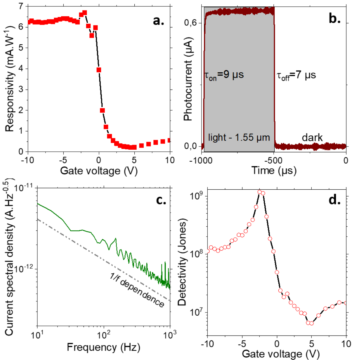
Figure 5 Infrared photodetection performance of the graphene/HgTe/graphene junction. a. Responsivity at 1.55 \mu\text{m} of the graphene/HgTe/ graphene junction, as a function of the applied gate bias. b. Temporal response of the graphene/HgTe/ graphene junction, under -1 V of gate bias. Dynamics appears to be limited by experimental setup. c. Current spectral density as a function of signal frequency, under -2.5 V of gate bias. The noise appears to be 1/f limited. d. Detectivity ( ie signal to noise ratio) at 1 kHz and 220 K as a function of the applied gate bias for the graphene/HgTe/ graphene junction.
