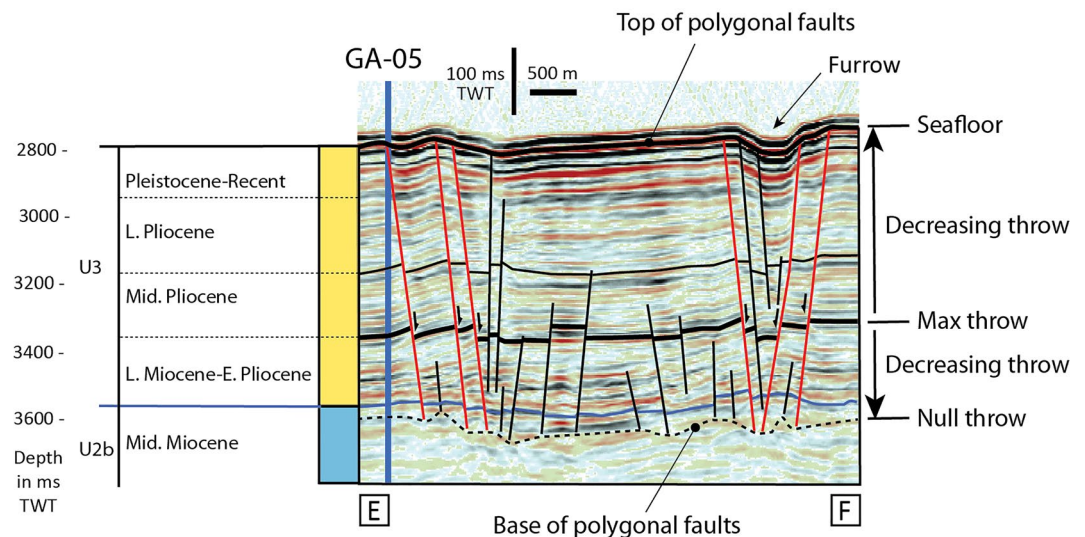
Figure 4. Detailed view of seismic profile GA-05 displaying decreasing offsets along fault planes both upward and downward. The maximum throw is located at the transition between Early and Middle Pliocene all over the Grenada Basin. Units were correlated and described in Garroq et al. (2021).
