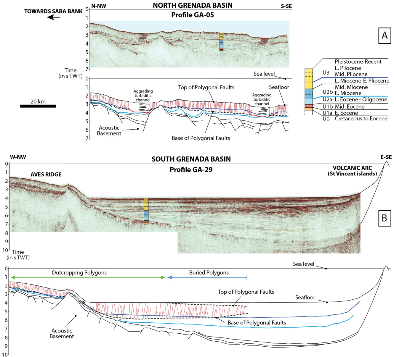
Figure 8. (a) Seismic profile GA-05 and its line-drawing displaying PFS in the NGB. The polygonal faults do not develop where deep aggrading turbiditic channels are present. PFS is getting thicker southward affecting almost all unit U2. Units U0 to U3 were correlated on GARANTI seismic data from previous studies and ODP/DSDP wells (Garroq et al., 2021); (b) seismic profile GA-29 and its line-drawing displaying PFS in the SGB. In both the western part of the SGB and the Aves Ridge, PF are reaching the seafloor. The base of PFS varies from west to east generally affecting the top of U2. In the eastern part of the SGB PFS is thinning eastward (both the top and the base of PFS are crosscutting stratigraphic horizons) and abruptly ends 40–70 km off the volcanic arc.
