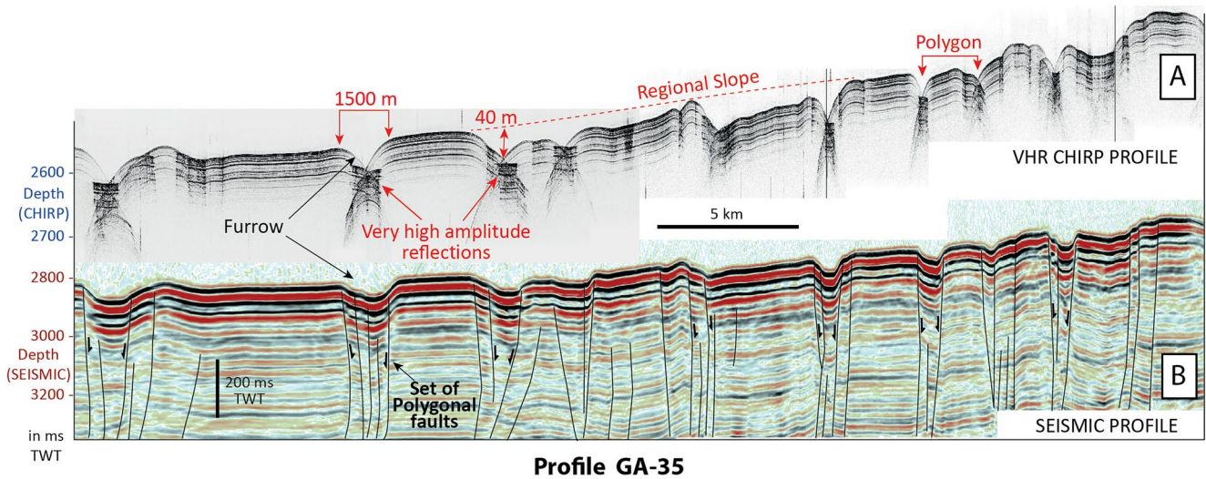
Figure 3. Very high-resolution seismic profile (CHIRP) at the identical horizontal scale than the corresponding seismic profile GA-35. The furrows are affecting the present-day seafloor and they are ~1,500 m wide and ~40 m deep (calculated with a velocity of 1,500 m/s in water). The difference in time arrival at the seabed between CHIRP and SEISMIC profiles comes from the acquisition. The seabed furrows represent the top of an underlying polygonal fault system. The bottom of furrows is characterized by very high amplitude reflections compared to well-bedded horizons between furrows.
