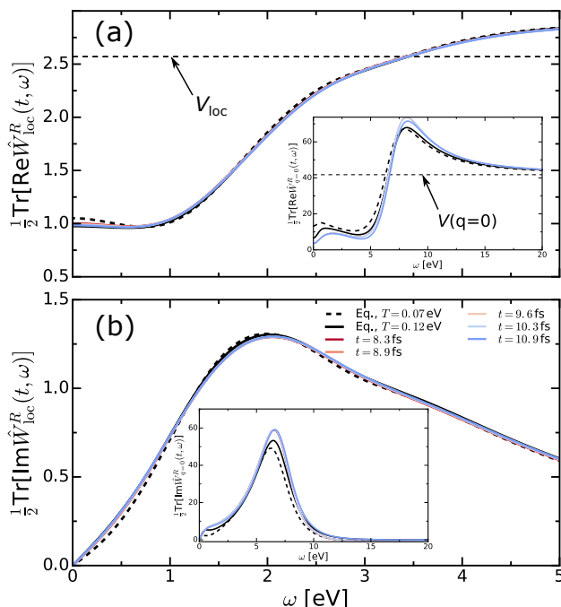
Figure 7: Time-dependent (a) real and (b) imaginary part of the local screened interaction W(\omega) after a photo-excitation. The equilibrium results at the initial T = 0.07 and the temperature of the thermalized system ( T = T_{\text{eff}} = 0.12 ) are shown by dashed and solid black lines, respectively. In the main panels, the blue lines are on top of the solid black lines.
