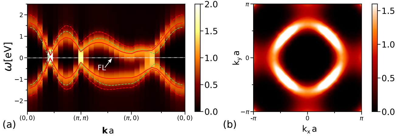
Figure 3: (a) \mathbf{k} -dependent band dispersion A_{\mathbf{k}}(\omega) for BaNiS 2 calculated for T = 0.07 eV on a 20 \times 20 \mathbf{k} grid. For the Fourier transformation we use a time window t_{\max} = 6.8 fs. The intensity is measured in units 1/\text{eV} . The red dashed line represents the Hartree-Fock contributions to the band structure, while the solid red line shows the QPGW band structure defined by Eq. (20). For comparison, we also show the non-interacting band dispersion by the green dashed line. The horizontal dashed line corresponds to the Fermi level FL. (b) A_{\mathbf{k}}(\omega = 0) plotted in the first Brillouin zone, showing the four Dirac points (surrounded by high intensity regions) on the diagonals. The intensity is measured in units 1/\text{eV} .
