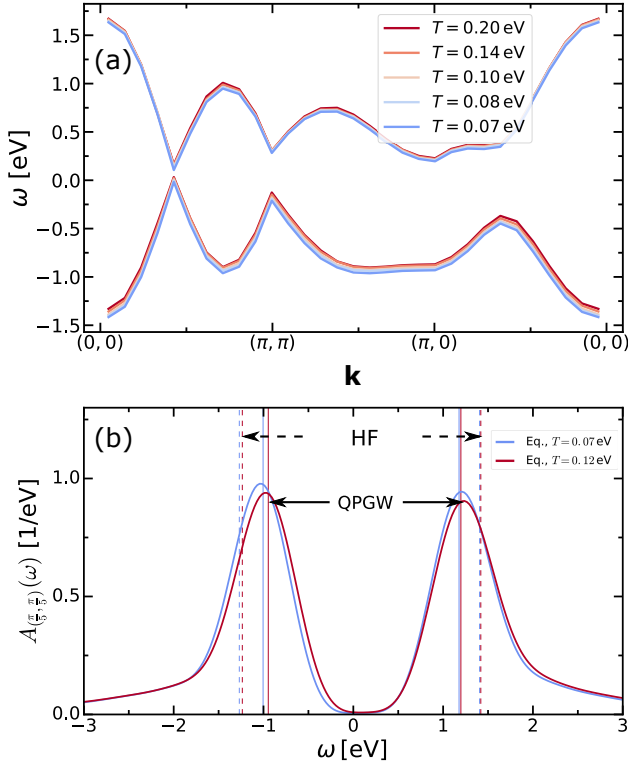
Figure 11: (a) Temperature dependence of the QPGW band structure calculated from Eq. (20). (b) \mathbf{k} -resolved spectral function calculated at \mathbf{k}\mathbf{a} = (\pi/5, \pi/5) for T = 0.07 eV (blue line) and T = 0.12 eV (red line).
