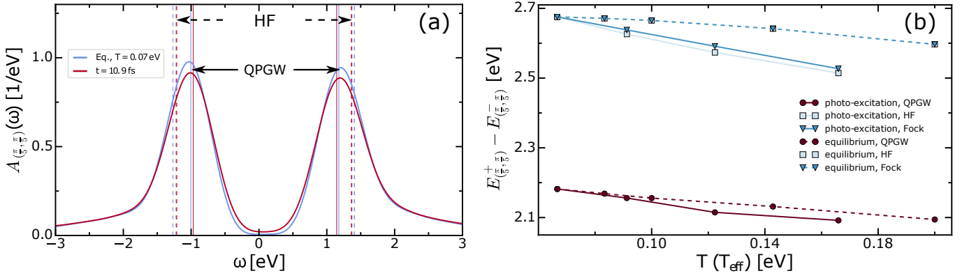
Figure 9: (a) Time-dependent \mathbf{k} -resolved spectral function calculated at (\mathbf{k}a = (\pi/5, \pi/5)) . The blue line corresponds to the equilibrium spectrum at T = 0.07 eV and the red line to the nonequilibrium spectrum after the pulse at t \approx 10.9 fs. Solid (dashed) vertical lines indicate the positions of the QPGW bands (bands which take into account the Hartree-Fock contribution to the full GW self-energy). (b) Difference between the QPGW energies of the upper (“+”) and lower (“-”) band at \mathbf{k}a = (\pi/5, \pi/5) in equilibrium (dark red dashed line with dots) and after a photo-excitation (dark red solid line with dots) as a function of T or T_{\text{eff}} . In addition, we plot the analogous results taking into account only the Fock (blue lines with triangles) and Hartree-Fock (light blue lines with squares) contributions to the full GW self-energy. The effective temperature after the photo-excitation is estimated from the total energy.
