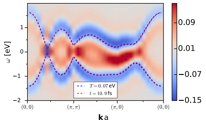
Figure 8: Difference \Delta A_k between the spectral function of the photo-excited system ( t \approx 10.9 fs) and the initial equilibrium spectral function ( T = 0.07 eV). The dashed lines indicate the QPGW peak positions from Eq. (20) for the initial equilibrium state (blue dashed line) and after the photo-excitation (red dashed line). Both spectral functions are calculated with t_{\text{max}} = 6.8 fs.
