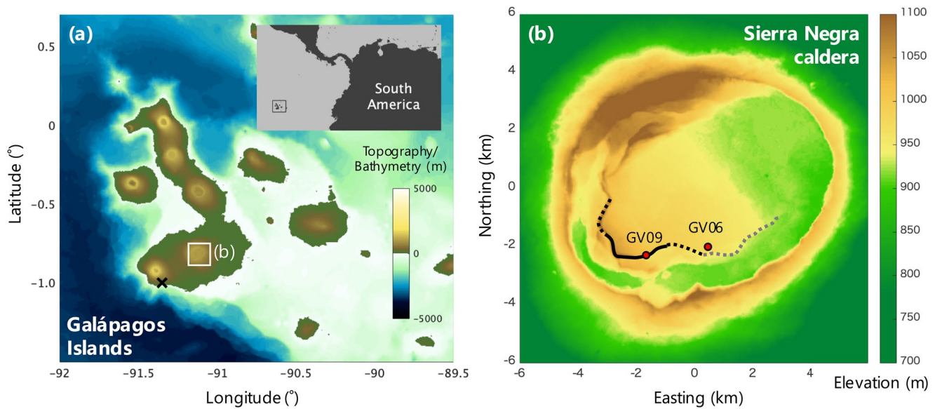
Figure 5. (a) Map of the Galápagos Islands. Topographic and bathymetric data are from GEBCO_2020. The black rectangle in the inset panel indicates the area shown in (a). The black cross represents the centroid location of the vertical-T earthquake of October 22, 2005, reported in the GCMT Catalog. (b) Map of the Sierra Negra caldera. Topographic data is from the Advanced Land Observation Satellite (ALOS) World 3D–30 m DEM (AW3D30) provided by the Japan Aerospace Exploration Agency (JAXA) (e.g., Tadono et al., 2014). The black curve indicates the fresh vertical scarp identified by Geist et al. (2008) during a field survey in June 2006; the part represented by the solid curve was clearly identified, whereas those along the dotted curves were less clearly defined. The red circles represent the locations of GPS stations used by Bell et al. (2021). The gray dotted curve indicates a possible geometry inferred in this study for the 2018 vertical-P earthquake (see Section 3.4).
