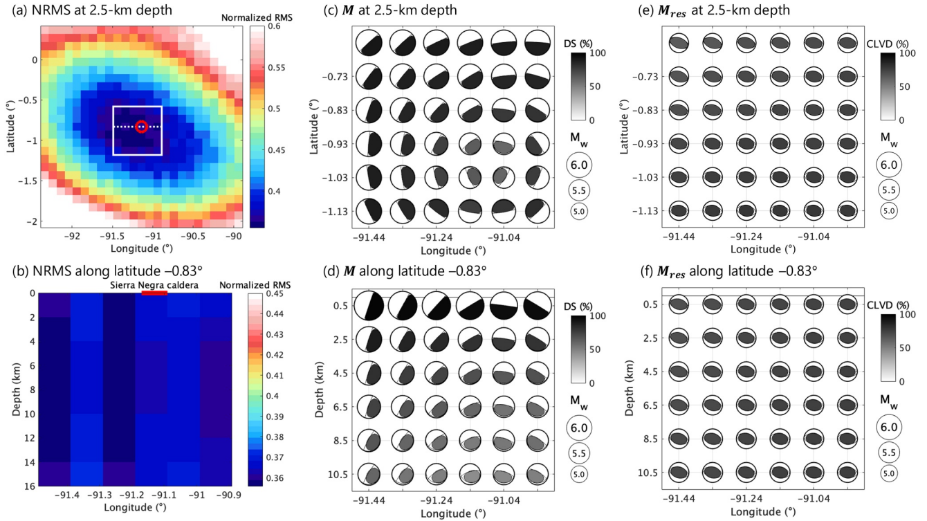
Figure 7. MT inversion for the vertical-T CLVD earthquake of October 22, 2005 at the Sierra Negra caldera. (a, b) Global NRMS misfits \rho of MT solutions at source locations distributed on (a) the x - y plane at a depth of 2.5 km in the crust and (b) the x - z plane along a latitude of 0.83^\circ (dashed white line in [a]). The red circle in (a) and the red line in (b) represent the approximate locations of the Sierra Negra caldera. (c, d) MT solutions at different centroid locations on (c) the x - y plane around the caldera (in the area shown by the white rectangle in [a]) and (d) the x - z plane. (e and f) Resolvable MTs on (e) the x - y plane around the caldera and (f) the x - z plane. All focal mechanisms are shown by projection of the lower focal hemisphere. In (b, d, and f), the vertical axis represents the centroid depth in the crust.
