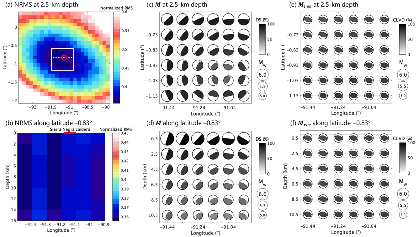
Figure 7. MT inversion for the vertical-T CLVD earthquake of October 22, 2005 at the Sierra Negra caldera. (a, b) Global NRMS misfits \rho of MT solutions at source locations distributed on (a) the x - y plane at a depth of 2.5 km in the crust and (b) the x - z plane along a latitude of 0.83^\circ (dashed white line in [a]). The red circle in (a) and the red line in (b) represent the approximate locations of the Sierra Negra caldera. (c, d) MT solutions at different centroid locations on (c) the x - y plane around the caldera (in the area shown by the white rectangle in [a]) and (d) the x - z plane. (e and f) Resolvable MTs on (e) the x - y plane around the caldera and (f) the x - z plane. All focal mechanisms are shown by projection of the lower focal hemisphere. In (b, d, and f), the vertical axis represents the centroid depth in the crust.
