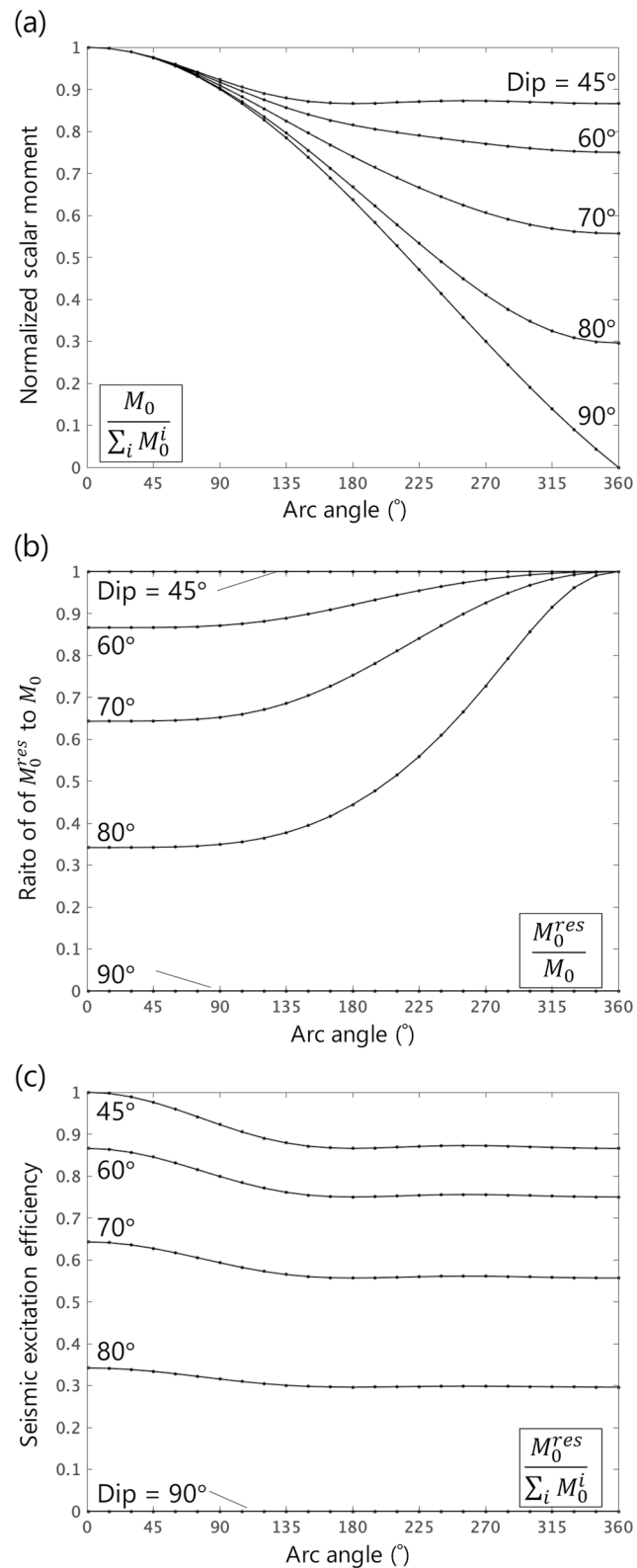
Figure 11. Seismic excitation efficiency of ring-faulting at a shallow source depth. (a) Geometrical cancellation of the scalar moment of idealized ring-faulting, calculated using Equation 13. (b) The ratio of M_0^{res} to M_0 of idealized ring-faulting, calculated using Equation 14. (c) The combined effect of (a) and (b), calculated using Equation 15.
