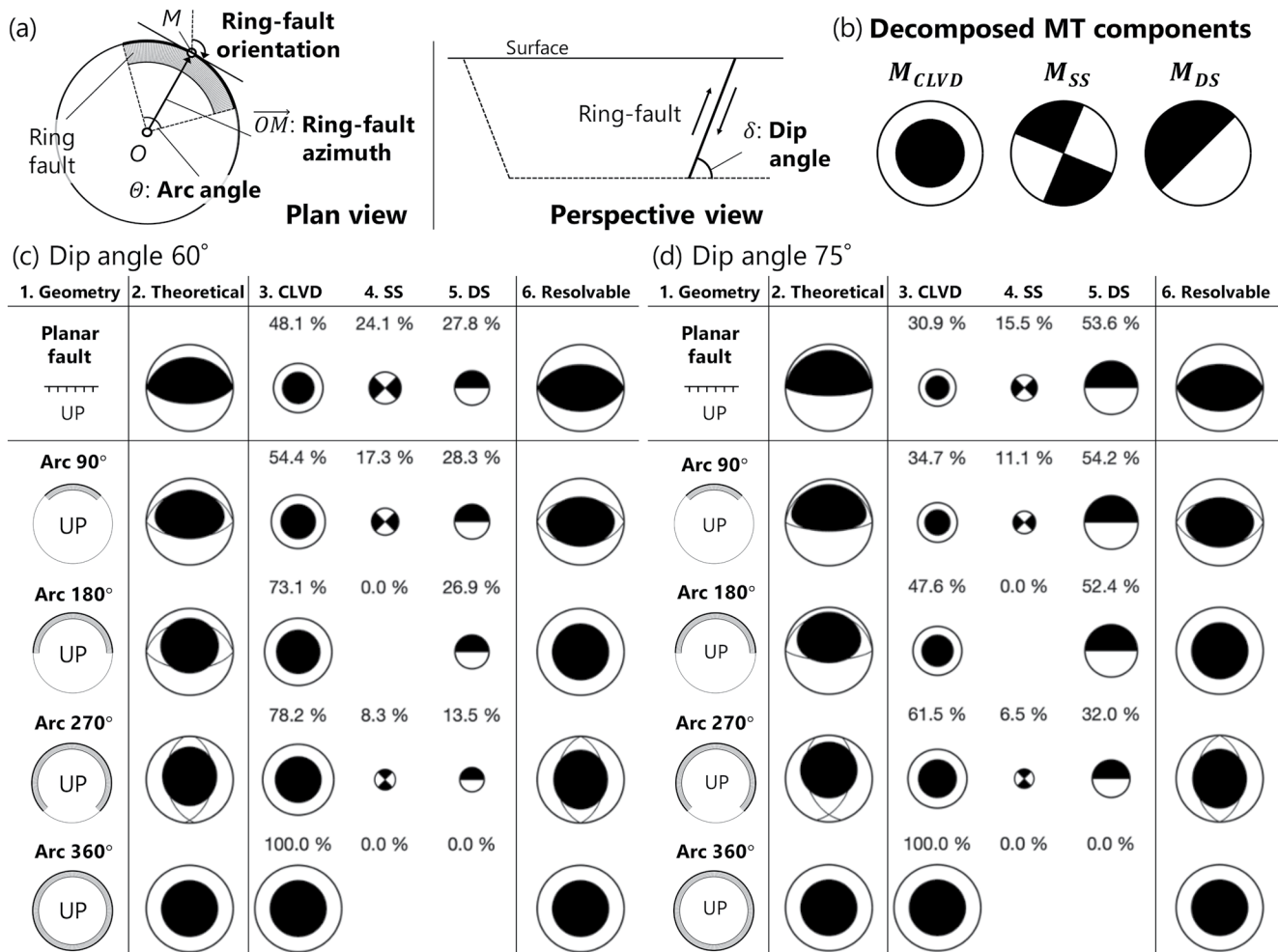
Figure 2. Modeling and decomposition of theoretical moment tensors of idealized ring-faulting. (a) Ring-fault parameters. Thick and thin arc curves represent up-dip and down-dip ends, respectively. Arc angle \Theta , dip angle \delta , and ring-fault azimuth OM are variable parameters. The ring-fault orientation is perpendicular to the ring-fault azimuth. The dip angle is uniform along the ring fault. (b) Three decomposed moment tensor (MT) components. (c)–(d) Theoretical MTs of ring-faulting with arc angles of 90°, 180°, 270°, and 360° and with dip angles of (c) 60° and (d) 75°. For reference, an MT of a planar faulting is also shown in the top row. Columns: (1) kinematics and geometry of ring-faulting, (2–6) focal mechanism diagrams of (2) the theoretical MT, (3–5) decomposed MT components (CLVD, SS, and DS) with their ratios, and (6) resolvable MT. The orientation of the best double-couple solution is shown by thin curves in columns 2 and 6. All focal mechanisms are shown by projection of the lower focal hemisphere. The diameter of the focal mechanism diagram is proportional to its scalar moment but slightly exaggerated for the component with percentages of < 10% for clear visualization.
