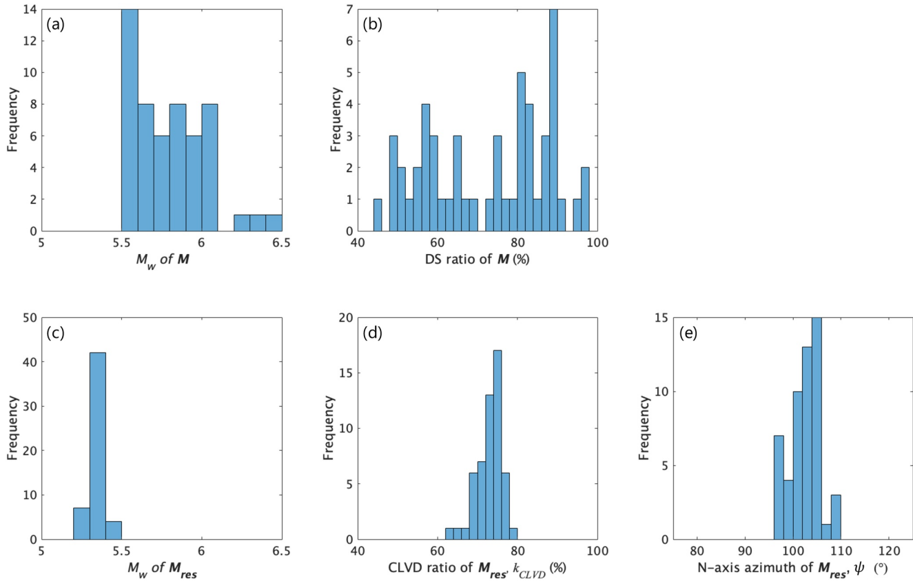
Figure 8. Histograms of the parameters of acceptable MT solutions. (a) M_w and (b) the ratio of the DS component of the acceptable MT solutions. (c) M_w of M_{res} , (d) the CLVD ratio k_{CLVD} , and (e) the N -axis azimuth \psi of M_{res} extracted from the acceptable MT solutions.
