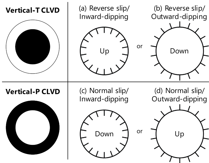
Figure 1. Two types of vertical-CLVD earthquakes caused by ring-faulting. (a–d) The kinematics and geometry of ring-faulting corresponding to the two endmembers of vertical-CLVD earthquakes (shown on the left). The circle represents the up-dip end of the ring fault, with short lines indicating the dip direction to the down-dip end. The direction of motion of the central block is indicated at the center of the circle.
