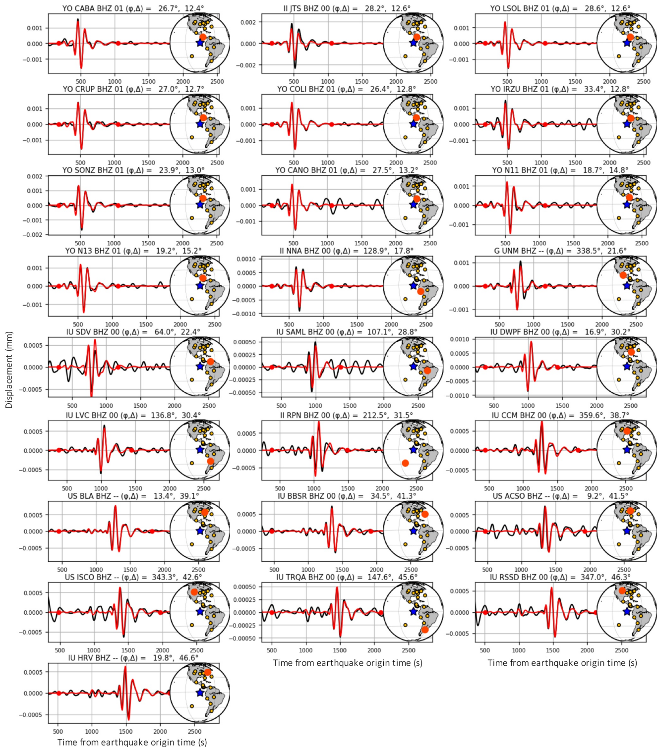
Figure 6. Model performance of MT inversion for the M_w 5.5 vertical-T CLVD earthquake of October 22, 2005. Red and black lines represent synthetic and observed waveforms, respectively. The start and end points of the inversion time window are indicated by red circles. In each inset map, the blue star and the large red circle represent locations of the epicenter ( 0.83^\circ\text{S} , 91.14^\circ\text{W} ) and the station. The station azimuth ( \phi ) and epicentral distance ( \Delta ) are indicated at the top of each panel.
