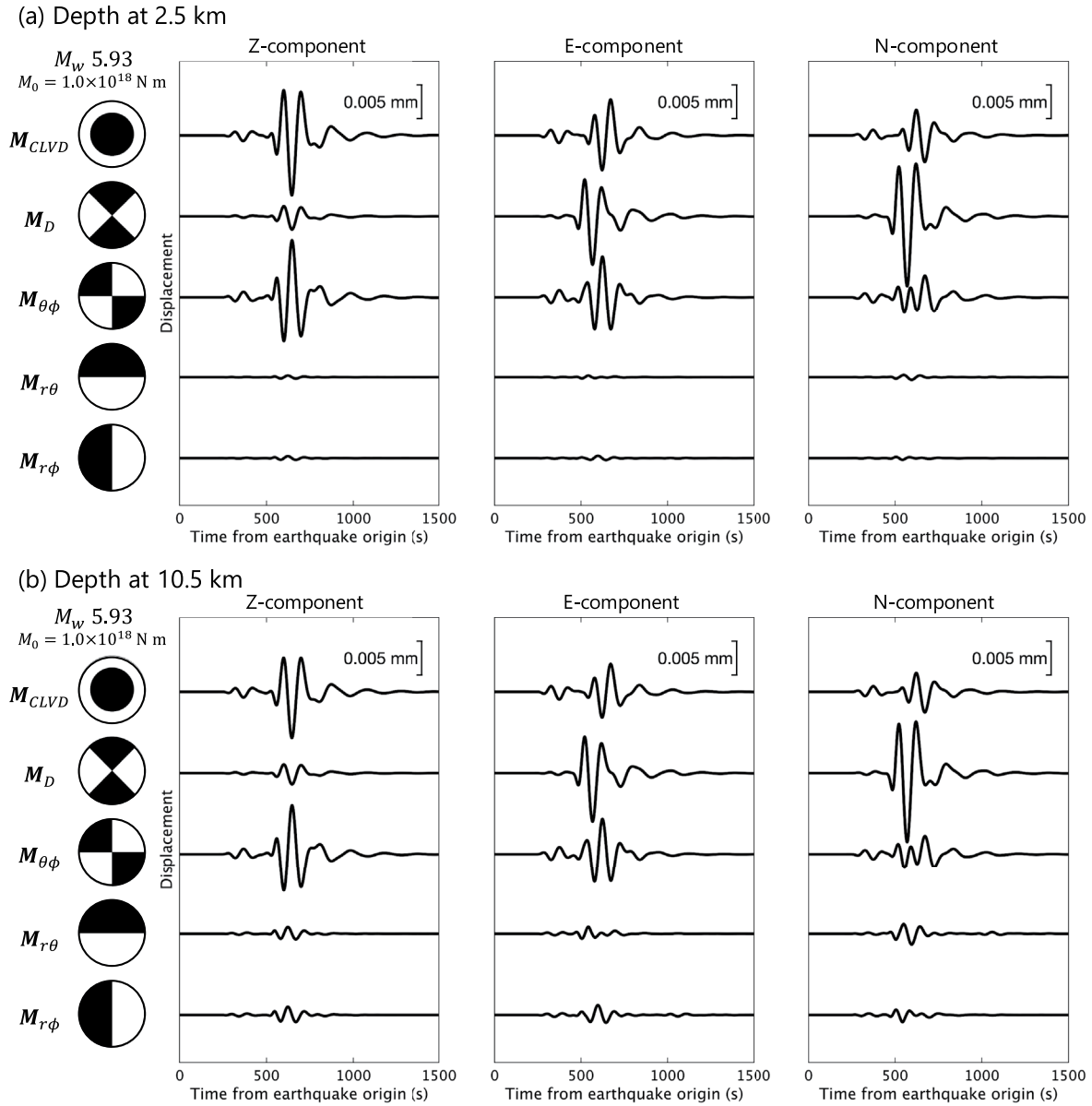
Figure 3. Synthetic long-period seismic waveforms from sources representing five elementary moment tensor components. The centroid depth is (a) 2.5 km and (b) 10.5 km in the crust. M_D and M_{\theta\phi} determine the SS component, and M_{r\theta} and M_{r\phi} determine the DS component. The virtual station is located at (\varphi, \Delta) = (19.2^\circ, 17.8^\circ) , where \varphi is the station azimuth from the north (eastward positive), and \Delta is the distance from the source. We use the W-phase code (Duputel et al., 2012; Hayes et al., 2009; Kanamori & Rivera, 2008) for the convolution of Green's functions and filtering. Green's functions are computed by the normal mode method (e.g., Takeuchi & Saito, 1972), with the 1-D Preliminary Reference Earth Model (PREM; Dziewonski & Anderson, 1981). A one-pass and fourth-order Butterworth bandpass filter with corner frequencies of 0.005 and 0.0125 Hz is applied.
