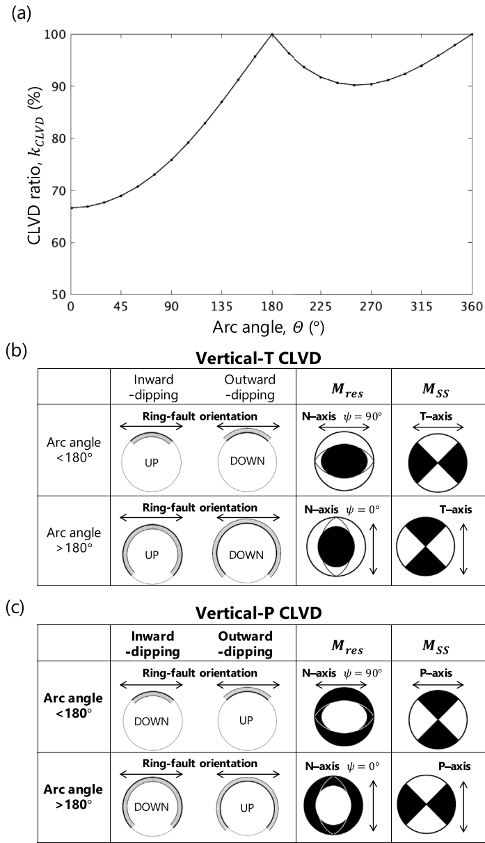
Figure 4. Relationship between M_{res} and ring-fault parameters. (a) The CLVD ratio, k_{CLVD} , of the resolvable MT, M_{res} , as a function of arc angle \Theta . Note that the relationship between k_{CLVD} and \Theta is independent of the dip angle of the ring fault. (b–c) Relationship between ring-fault geometry and M_{res} for (b) vertical-T earthquakes and (c) vertical-P earthquakes. In the second column, the dip direction of the ring fault (inward or outward), the kinematics of the central block (up or down), and the ring-fault orientation (an arrow) are shown. In the third column, M_{res} is shown with the orientation of its N-axis (arrow). In the fourth column, the SS component is shown with its T-axis or P-axis (arrow). Note that the N-axis of M_{res} is the same as the T- and P-axis of the SS component for vertical-T and vertical-P earthquakes, respectively.
