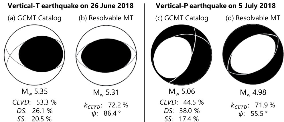
Figure 10. GCMT solutions for two vertical-CLVD earthquakes during the 2018 volcanic activity. (a) MT solution with the ratios of the three MT components and (b) resolvable MT of the M_w 5.3 earthquake of June 26, 2018 with the ratio of the CLVD component k_{CLVD} and the N -axis azimuth \psi obtained from the GCMT Catalog. (c, d) The same as (a, b) but for the M_w 5.1 earthquake of July 5, 2018. All focal mechanisms are shown by projection of the lower focal hemisphere.
