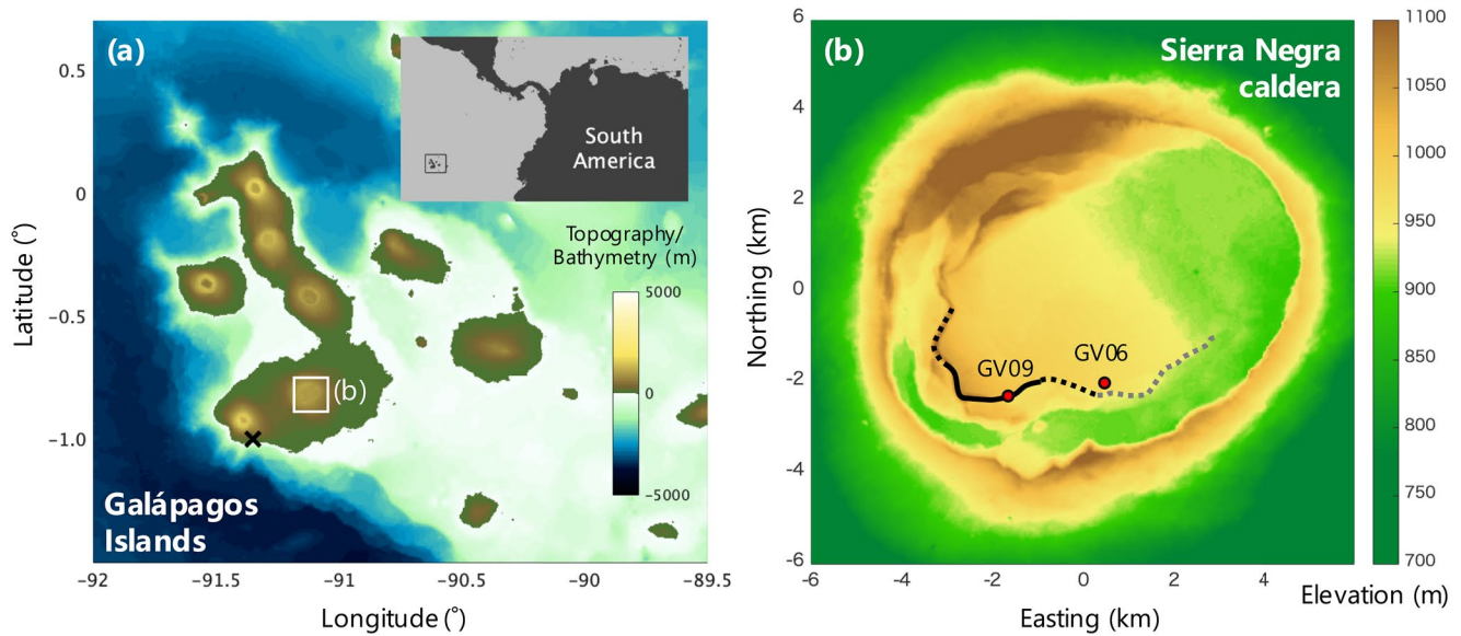
Figure 5. (a) Map of the Galápagos Islands. Topographic and bathymetric data are from GEMBCO_2020. The black rectangle in the inset panel indicates the area shown in (a). The black cross represents the centroid location of the vertical-T earthquake of October 22, 2005, reported in the GCMT Catalog. (b) Map of the Sierra Negra caldera. Topographic data is from the Advanced Land Observation Satellite (ALOS) World 3D–30 m DEM (AW3D30) provided by the Japan Aerospace Exploration Agency (JAXA) (e.g., Tadono et al., 2014). The black curve indicates the fresh vertical scarp identified by Geist et al. (2008) during a field survey in June 2006; the part represented by the solid curve was clearly identified, whereas those along the dotted curves were less clearly defined. The red circles represent the locations of GPS stations used by Bell et al. (2021). The gray dotted curve indicates a possible geometry inferred in this study for the 2018 vertical-P earthquake (see Section 3.4).
