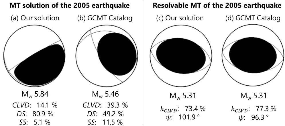
Figure 9. MT solutions and resolvable MTs of the M_w 5.5 vertical-T CLVD earthquake of October 22, 2005. (a) MT solution with the ratios of the three MT components and (c) resolvable MT with the ratio of the CLVD component k_{CLVD} and the N -axis azimuth \psi obtained from our MT inversion at a depth of 2.5 km in the crust just below the caldera. (b) MT and (d) resolvable MT obtained from the GCMT Catalog. All focal mechanisms are shown by projection of the lower focal hemisphere.
