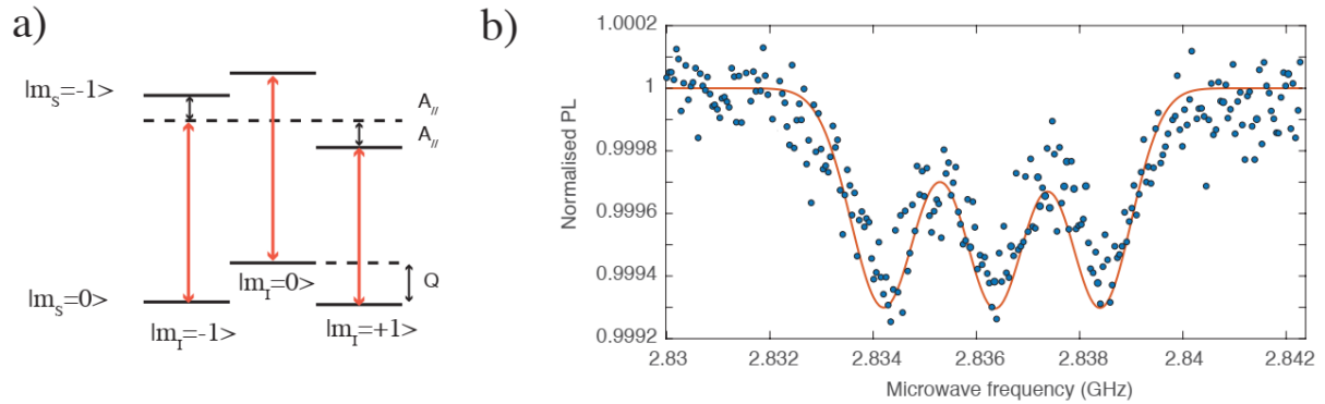
Fig. 11 (a) Energy level scheme of the NV centre showing the 3 main transitions due to hyperfine splitting induced by ^{14}\text{N} . (b) Electronic spin resonance spectrum on one of the NV orientations in the irradiated sample (A).
