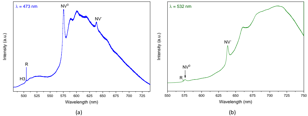
Fig. 2. PL spectra of as-grown freestanding CVD diamond with N 2 O addition (sample A) under (a) 473 nm and (b) 532 nm excitation lines respectively. The diamond Raman peak is labelled R and the main emissions are indicated.
