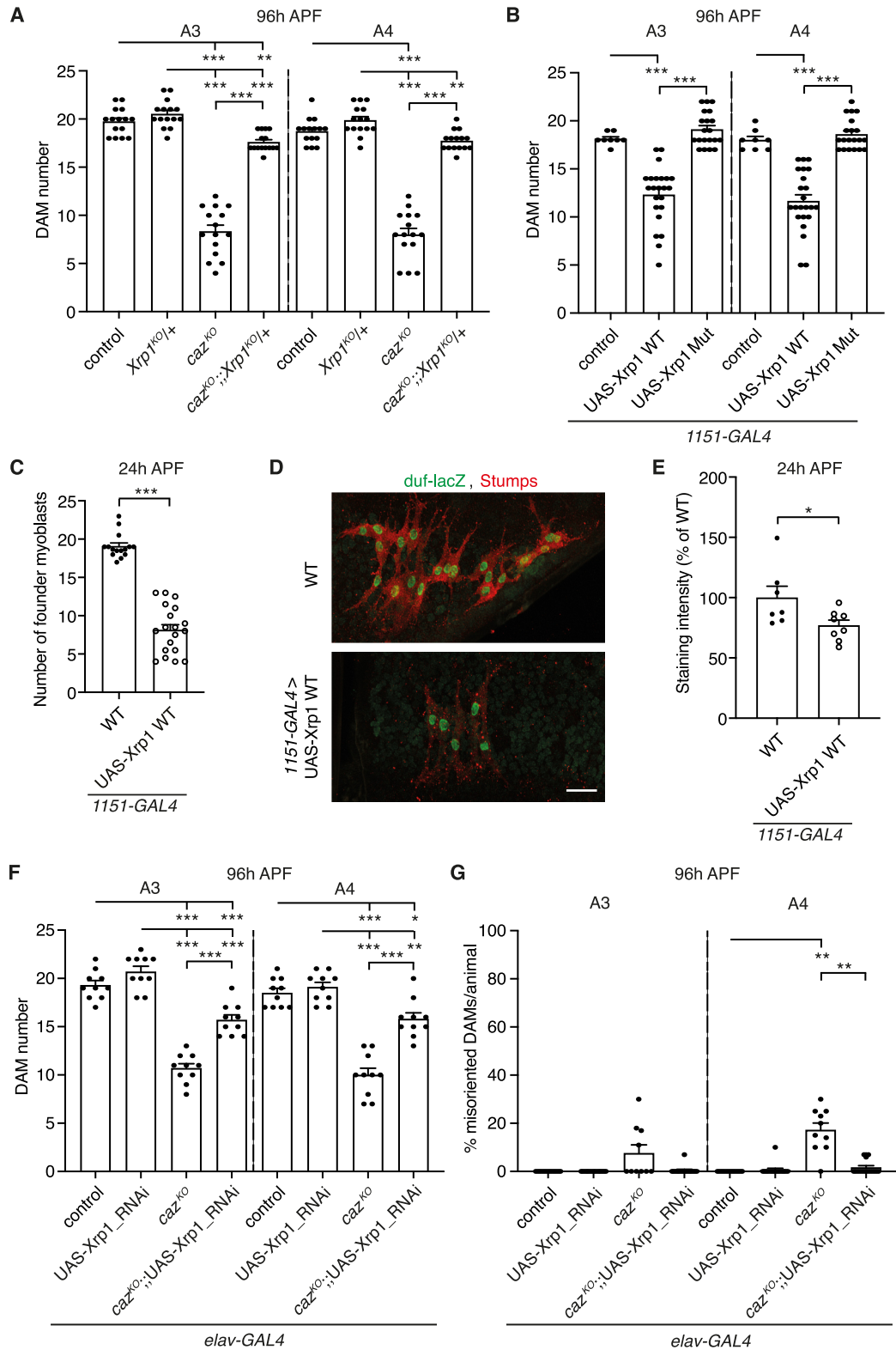
Fig 6. Increased Xrp1 levels mediate caz mutant muscle phenotypes. A, Quantification of DAM number in segments A3 and A4 of 96 h APF caz KO pupae that are heterozygous for Xrp1 KO ( caz KO /Y; Mhc-GFP,his-RFP/+; Xrp1 KO /+ ) as compared to the relevant control genotypes (+/Y; Mhc-GFP,his-RFP/+ // +/Y; Mhc-GFP,his-RFP/+; Xrp1 KO /+ // caz KO /Y; Mhc-GFP,his-RFP/+ ). Two-way
