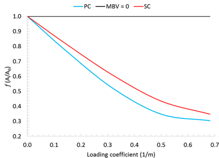
Figure 14. Impact of exposed surface area on indoor RH variation for PC and SC.
