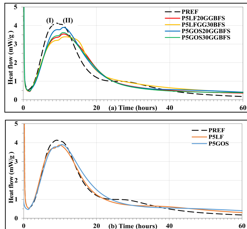
Figure 2. Heat flow of (a) ternary cement pastes; (b) binary cement pastes.
