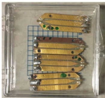
Figure 4. The microfabricated GSG probes mounted onto PCB for DC characterization.
