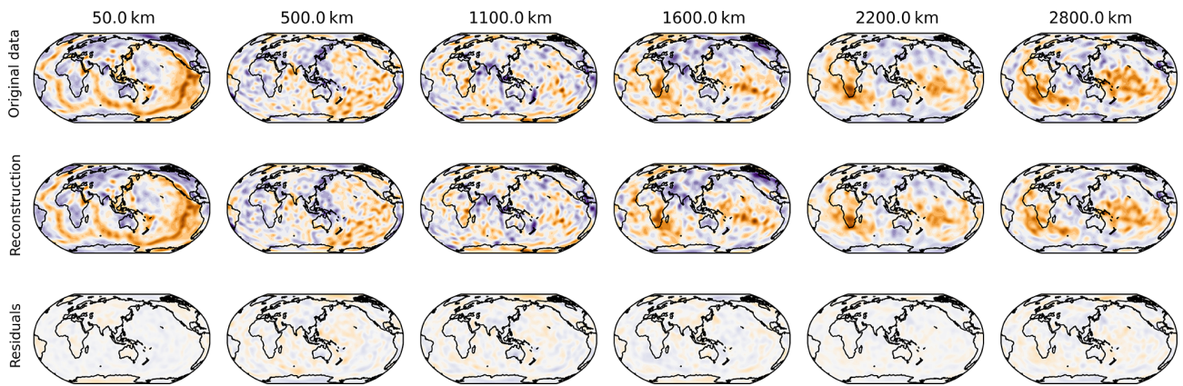
Figure B1. Examples of six depth slices in the original SEMUCB–WM1i model (top), in the model recovered without the principal components with less than 1% of the variance, i.e. with nine components (middle), and differences between the two (bottom).
