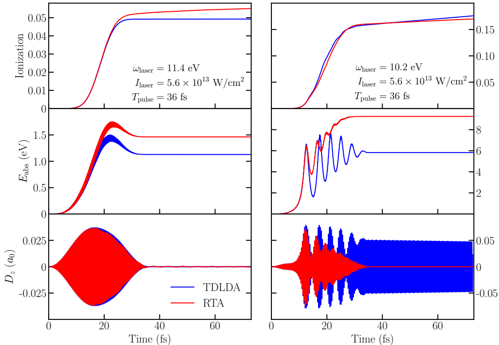
Figure 13: Comparison of TDLDA (blue) and RTA (red) time evolution of three basic observables for \text{H}_2\text{O} : dipole moment perpendicular to molecular plane (bottom), absorbed energy (middle) and total ionization (top). The water molecule was excited by a laser pulse with frequency \omega_{\text{laser}} = 11.4 eV for the off-resonance case (left column) and \omega_{\text{laser}} = 10.2 eV for the on-resonance case (right column). For both frequencies, the laser intensity is I = 5.6 \times 10^{13} \text{ W/cm}^2 , and the total pulse length T_{\text{pulse}} = 36 fs. The water molecule is in the xy plane and the laser polarization is along z , see inset of figure 8.
