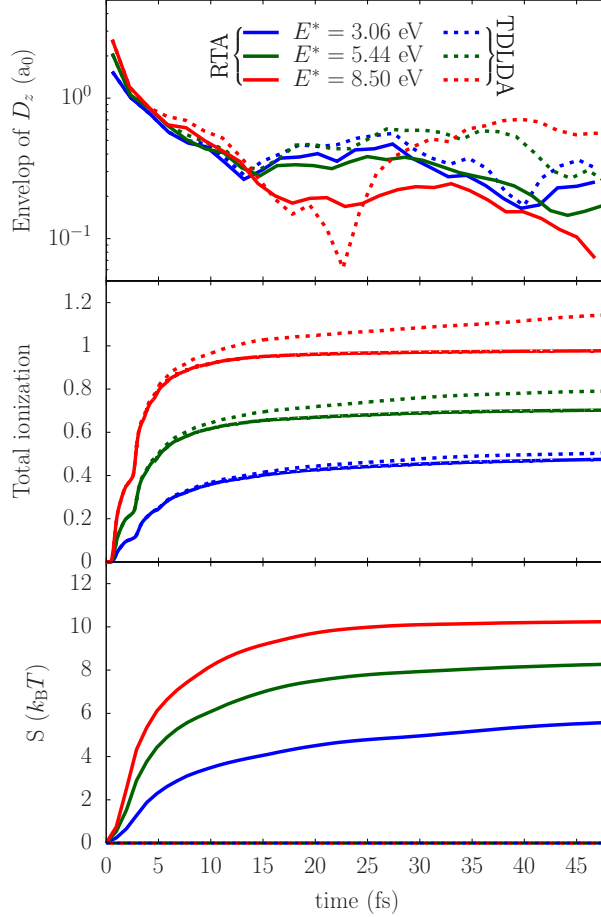
Figure 12: Time evolution of the one-body entropy (bottom), the total ionization (middle) and the envelope of the dipole moment in z direction (top, vertical log scale) of \text{Na}_{11}^+ after various initial boosts delivering different excitation energies E^* as indicated. Full curves are obtained in RTA while dashed curves are obtained with TDLDA.
