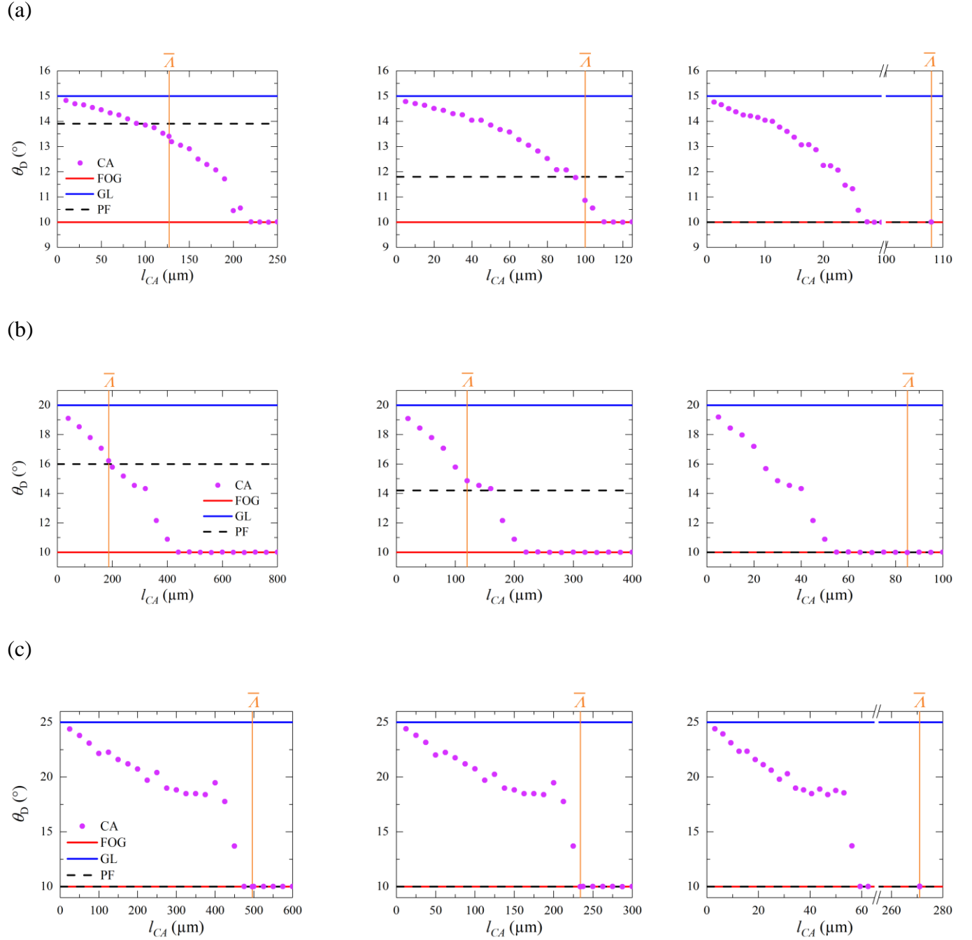
Fig. 15. Evolution of the diverging GB angle, \theta_D , in CA simulations (purple symbols). The crystal axis angle of grain 1, \alpha_1 , is equal to (a) 20^\circ , (b) 30^\circ and (c) 40^\circ with the angle of grain 2 \alpha_2 fixed at 10^\circ . Three temperature gradients are investigated: G = 237.5 \text{ K m}^{-1} (first column), G = 475 \text{ K m}^{-1} (second column), and G = 1900 \text{ K m}^{-1} (third column). The solution corresponding to GL (resp. FOG) prediction is illustrated as the blue (resp. red) horizontal line. The average GB angle from PF prediction, \overline{\theta_D} , (Fig. 6a) is shown with the horizontal dashed black line. The position of the relevant length scale, \overline{\lambda} , bridging PF and CA (listed in Table 3) is illustrated with the vertical line.
