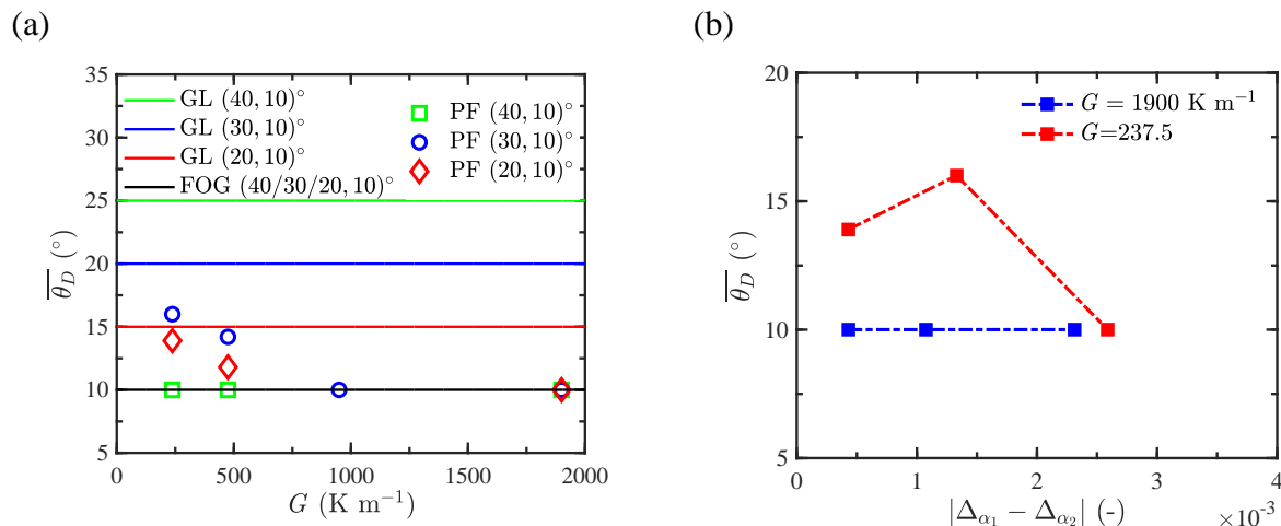
Fig. 6. Phase-field simulation results showing a transition from FOG to GL with decreasing temperature gradient. (a) Average diverging GB orientation angle, \overline{\theta}_D , vs G for different bi-crystallographies (20^\circ, 10^\circ) , (30^\circ, 10^\circ) and (40^\circ, 10^\circ) , and (b) \overline{\theta}_D , vs steady-state undercooling difference, |\Delta_{\alpha_1} - \Delta_{\alpha_2}| , in the FOG high-gradient ( G = 1900 \text{ K m}^{-1} ) and GL low-gradient ( G = 237.5 \text{ K m}^{-1} ) dominant regimes. Each point from left to right along the |\Delta_{\alpha_1} - \Delta_{\alpha_2}| axis corresponds to (20^\circ, 10^\circ) , (30^\circ, 10^\circ) , and (40^\circ, 10^\circ) , respectively.
