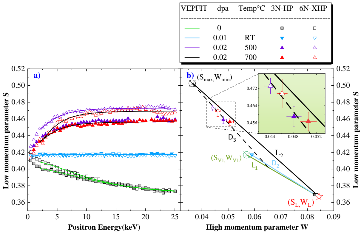
237 Figure 3: a: Low momentum annihilation fraction S as a function of positron energy and b: the fit extracted 238 values S as a function of the high momentum annihilation fraction W ones in 3N-HP W samples (solid symbols) 239 and 6N-XHP samples (open symbols), before irradiations (square ■(3N) □(6N)) after irradiation at room 240 temperature (0.01 dpa downward triangle ▼(3N) ▽(6N)), at high temperatures (upward triangle ▲(3N) 241 △(6N), plotted in purple for irradiation performed at 0.02 dpa, 500 °C, and in red for 0.02 dpa 700 °C)
