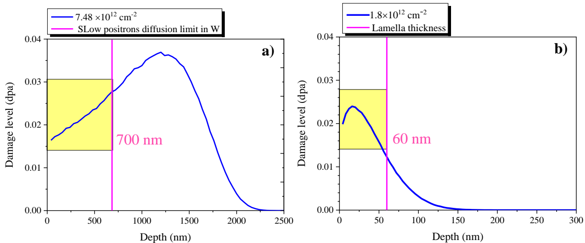
114 Figure 2 : a) Damage profile of self-irradiation with 7.48 \times 10^{12} \text{ W}^+ \cdot \text{cm}^{-2} ( 15^\circ , 20 MeV), b) damage profile of self- 115 irradiation with 1.8 \times 10^{12} \text{ W}^+ \cdot \text{cm}^{-2} ( 45^\circ , 1.2 MeV) according to SRIM2008 with Kinchin-Pease formalism. The 116 characterized region depends on the thickness that can be probed by slow positrons: at most 700 nm for 25 117 keV [36] for PAS measured samples and about 60 nm for TEM observed samples.
