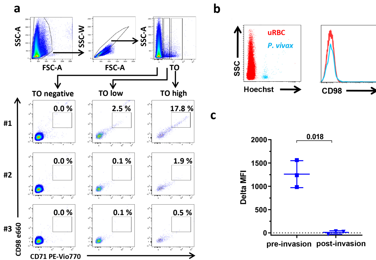
Extended Data Fig. 2 | Flow cytometry analysis of adult peripheral blood, cord blood and P. vivax isolates. a , Flow cytometry profile of CD98 and CD71 expression on thiazole orange (TO) negative, low and high erythrocytes for three different human adult peripheral blood samples (forward scatter (FSC) for x-axis and side scatter (SSC) for y-axis). The TO high subset represents the most immature reticulocyte population compared to low subset. b , Flow cytometry histogram of CD98 expression (right) at the surface of P. vivax rings, early infected reticulocyte forms, gated on Hoechst-positive cells (left), side scatter (SSC) for y-axis. The infected cells positive for Hoechst (a DNA stain) are in blue and the uninfected red blood cells (uRBC), which do not contain DNA, are in red. c , Comparison of delta of geometric mean fluorescence intensity (MFI) between immature reticulocytes from three cord blood samples and three vivax infected patients (ring stage), Values are expressed as mean \pm SD, unpaired Student t -test.
