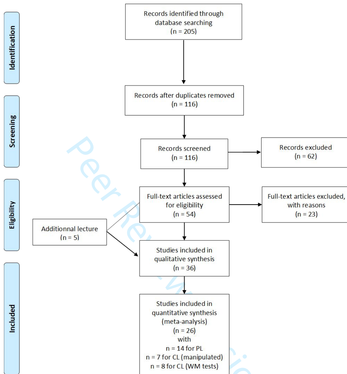
Figure 1: The PRISMA flow diagram (adapted from Moher et al., 2009) representing the number of studies included and excluded at each step of the qualitative and quantitative analysis. For the final step, we informed about the number of studies included in each of the three meta-analysis: the perceptual load (PL) or cognitive load (CL) effect on IB, with the latter investigated through direct manipulation or measured through working memory (WM) tests (e.g., OSPAN). However, note that the number of studies included in the meta-analysis was different (i.e., lower) than the number of entries (experiments and/or conditions) on which the meta-analysis relied on.
