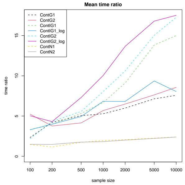
(b) Continuous distributions
