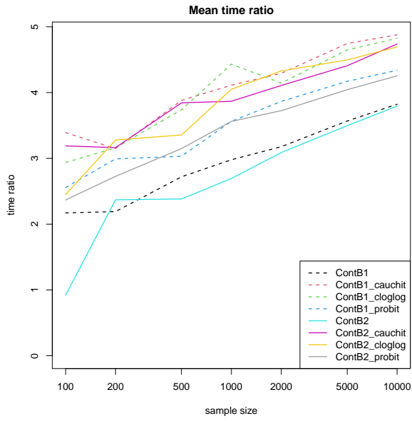
(a) Bernoulli distribution
