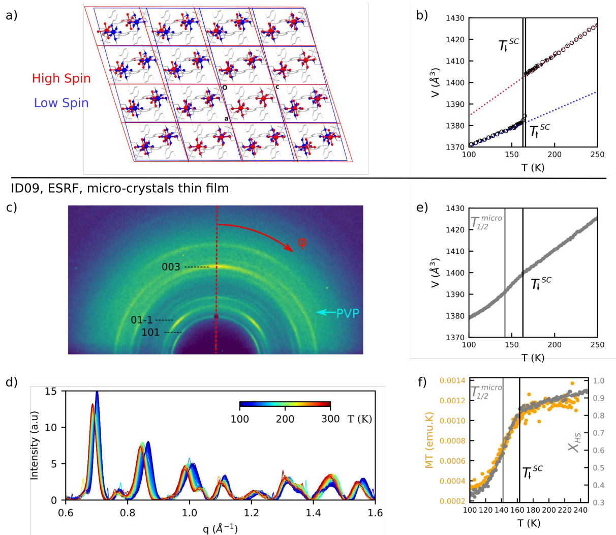
2 3 Figure 1. a) [\text{Fe}^{\text{III}}(3\text{-MeO-SalEen})_2]\text{PF}_6 molecular lattices in LS (100 K, blue) and HS (293 K, 4 red) state, shown in the (a, c) plane. Ligands (in gray) are shown for the LS structure only. b) 5 XRD measurement on a single crystal: temperature evolution of the unit cell volume ( T 6 decreasing, plain black triangles, T increasing, open circles) for extraction of thermal expansion 7 parameters of the HS (red dotted line) and LS (blue dotted line) unit cell (SI Method, 8 [Tissot2011]). Vertical black lines represent transition temperatures for T decreasing ( T_{\downarrow}^{\text{SC}} ) 9 and T increasing ( T_{\uparrow}^{\text{SC}} ). c) to f) Synchrotron x-ray powder diffraction on micro-crystals 10 measured at ESRF, ID9 beamline: c) Diffraction image measured at T = 293 K. d) 1D powder 11 patterns after azimuthal averaging of diffraction images (a) for the different temperature
