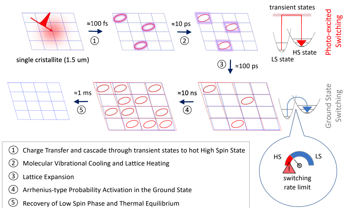
2 Figure 4. Photoexcitation cycle of a single crystallite upon spin-crossover. Top: laser induced 3 charge transfer promotes LS molecules (not shown for clarity) residing in LS lattice (blue) to 4 a hot HS state (shape and color coded consistently with figure 3) in less than 100 fs. Vibrational 5 cooling of hot molecules with LS lattice (color coded consistently with figure 3) takes place on 6 the picosecond time scale. Bottom: volume expansion of heated lattice in 100's ps, and 7 coexistence of LS molecules (not shown) in thermally dilated LS lattice (blue) with photo- 8 switched HS molecules (red) in thermally dilated HS lattice (red). HS and LS lattices 9 superimposed to emphasize their likely coexistence (only average volume measured with 10 XRD). Shift of the switching regimes: LS molecules residing in the ground state switch to the 11 HS state according to LS/HS occupancy probabilities modified by lattice expansion; the delay 12 between expansion (300 ps, or less for nano-crystallites) and the switching (ns time-scale), due 13 to incompressible Arrhenius-type kinetics sketched in the insert.
