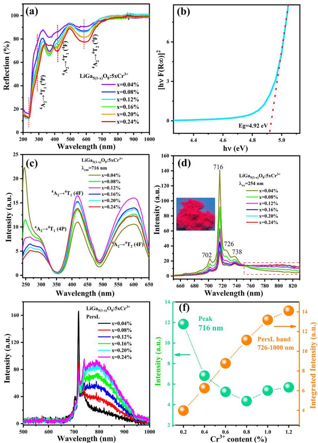
Fig. 3 Optical characteristics of \text{LiGa}_{5(1-x)}\text{O}_8:5x\text{Cr}^{3+} . (a) DR spectra. (b) The plot of [\text{F(R}\infty)\text{h}\nu]^2 versus energy (eV). (c) PLE ( \lambda_{\text{em}} = 716 nm) and (d) PL ( \lambda_{\text{ex}} = 254 nm) spectra. The inset of (d) is the image of sample x = 0.12\% under a 254 nm lamp. (e) PersL spectra recorded after irradiated by a 254 nm lamp for 30 s. (f) The peak PersL intensities of 716 nm and the PersL band (726-1000 nm) as a function of \text{Cr}^{3+}
