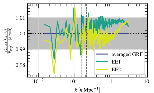
Figure 12. Comparison of EuclidEmulator1 and EuclidEmulator2 to the NLC computed from an ensemble average of 50 Gaussian random field simulations. It can be seen that the cosmic variance is responsible for the oscillatory peaky pattern in Fig. 11, as the vertical, black, dashed lines correspond to the two highlighted peaks in that figure.
