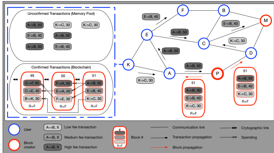
Fig. 3. Multi-Agent Representation of a Blockchain System [43].
