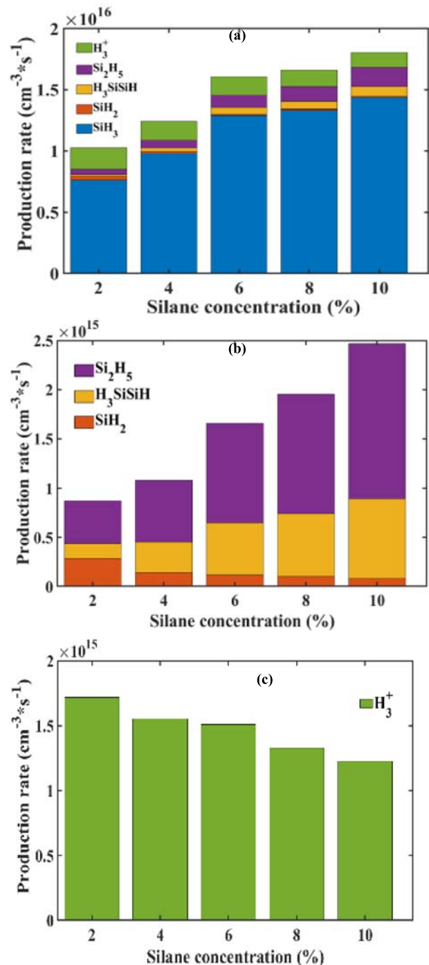
Figure 5. Computed time-space-averaged production rates of the species as a function of silane concentration: (a) SiH_2 , Si_2H_5 , H_3SiSiH , SiH_3 and H_3^+ ; (b) radicals SiH_2 , Si_2H_5 , and H_3SiSiH ; (c) H_3^+ ions.
