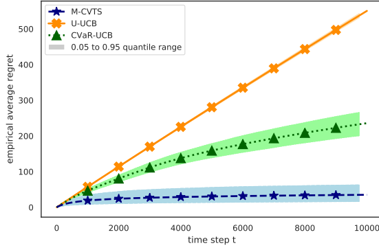
Figure 5: Experiment 1 with Multinomial arms, all algorithms, \alpha = 10\%
