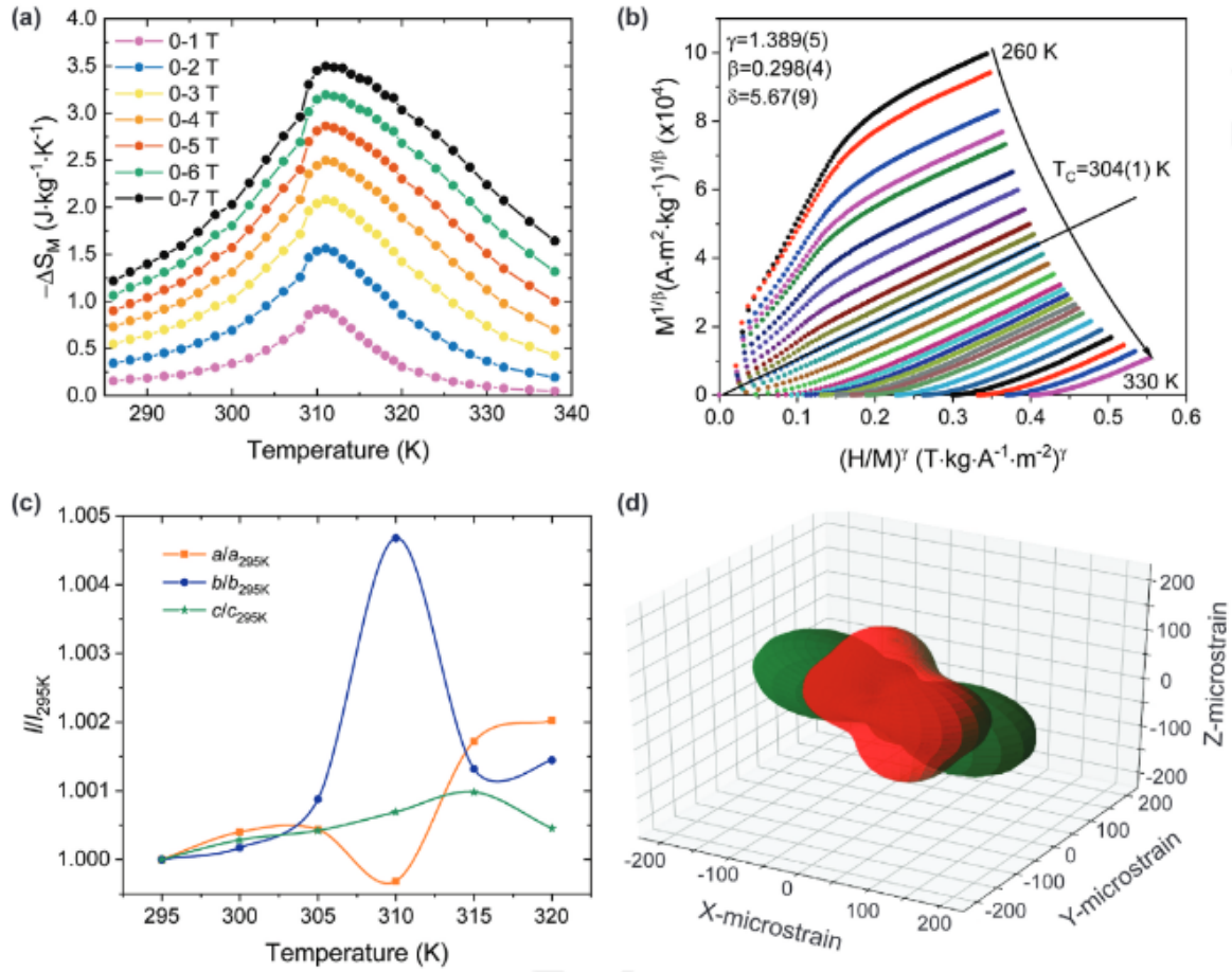
Figure 2. a) Magnetic entropy change ( \Delta S_M ) for MnZnSb between 285 and 340 K in magnetic field ranging from 1 to 7 T with a magnetic field independent \Delta S_M maximum observed at 310 K. b) Arrott-Noakes plot for the isothermal magnetization of MnZnSb measured between 260 and 330 K. The extracted critical exponents are \gamma=1.389(5) and \beta=0.298(4) with a T_C = 304 K (black straight line). c) Relative change of MnZnSb lattice parameters ( a -orange square, b -blue dots, and c -green stars. Lines are guides to the eyes) with respect to their 295 K value obtained from Le Bail fittings of temperature dependent PND using a triclinic cell. d) 3D representation of the strain tensor obtained from SXRD Le Bail fittings including anisotropic broadening below the T_C of MnZnSb (green) and above the T_C of Mn_{0.9}Fe_{0.1}ZnSb (red).
