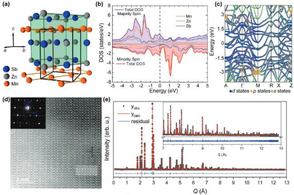
Figure 1. a) Prototypical structural model of the PbFCI structure for MnZnSb. The tetragonal unit cell is represented with the black cuboid. The structure is described by square net layers of Mn atoms (orange spheres) intercalated in a NaCl like blocks (green shaded cube) composed of Zn (grey spheres) and Sb (blue spheres) atoms. b) Total (purple-majority and red-minority spins) and atomic contributions (Mn-orange line, Zn-grey line, and Sb-blue line) spin-polarized density of states. c) Fat band electronic band structure along selected high symmetry directions with Mn d (blue), p (orange) and s (green) orbital projection for MnZnSb. Orbital character is used to distinguish between the flat bands (d states) and hybridized itinerant, broad bands (s-p states) about the Fermi level. d) [110] oriented HAADF image of a single MnZnSb grain with corresponding calculation and atomic projection (bottom right inset). The top left inset shows a corresponding electron diffraction pattern. e) Le Bail fitting (red line) of synchrotron X-ray diffraction data (black dots) using a triclinic MnZnSb cell with anisotropic strain broadening. The blue line represents the residual of the fit. The high Q region is shown in the inset.
