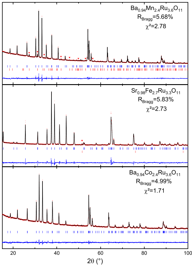
FIG. 2. Rietveld refinement of \text{Ba}_{0.94}\text{Mn}_{2.4}\text{Ru}_{3.6}\text{O}_{11} (upper panel), \text{Sr}_{0.98}\text{Fe}_{2.7}\text{Ru}_{3.3}\text{O}_{11} (middle panel), and \text{Ba}_{0.94}\text{Co}_{2.4}\text{Ru}_{3.6}\text{O}_{11} (bottom panel) with their respective quality factor. Red crosses are experimental data, black lines are calculated fits, and blue lines are the differences between fits and data. Note the presence of \text{BaRuO}_3 (red triangles) as impurity in \text{Ba}_{0.94}\text{Mn}_{2.4}\text{Ru}_{3.6}\text{O}_{11} , and Fe (red triangles) in \text{Sr}_{0.98}\text{Fe}_{2.7}\text{Ru}_{3.3}\text{O}_{11} .
