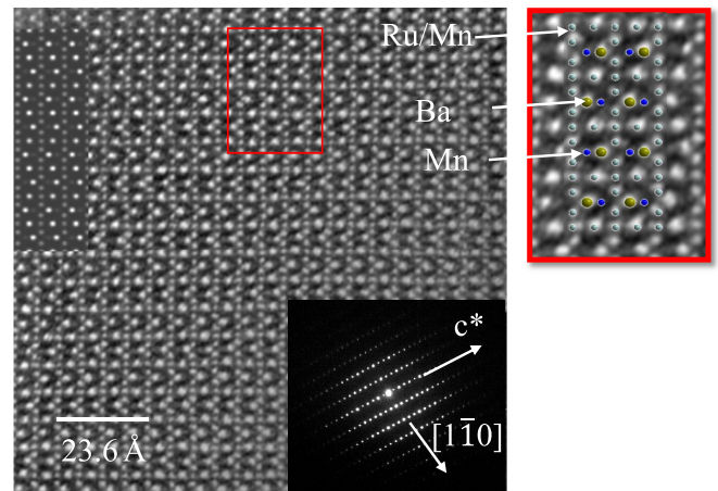
FIG. 3. Crystal model and STEM ADF image of \text{Ba}_{0.94}\text{Mn}_{2.4}\text{Ru}_{3.6}\text{O}_{11} (left panel) with ED pattern (left panel bottom inset), simulation (left panel upper inset), and superposition of the crystallographic structure extracted from Rietveld refinements with atom in color (gray: Ru/Mn in 4e and 6g sites, blue: Mn in 2d sites, and yellow Ba in 2a sites).
