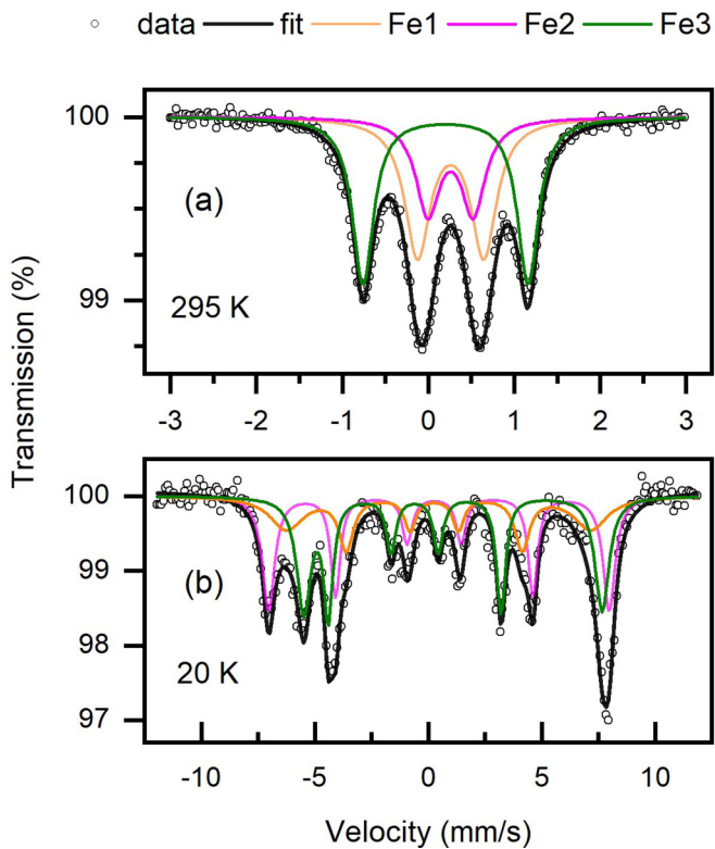
FIG. 4. Mössbauer spectra of \text{Sr}_{0.98}\text{Fe}_{2.7}\text{Ru}_{3.3}\text{O}_{11} at 295 K (a) and 20 K (b). The spectra were decomposed into three subspectra corresponding to the Fe1 (orange), Fe2 (pink), and Fe3 (green) sites where the iron cations are positioned.
