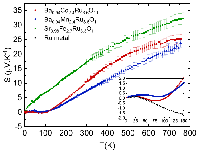
FIG. 11. Temperature-dependent Seebeck coefficient. Inset: low-temperature S(T) of Co-, and Mn- 124 oxides and Ru metal, from 8 to 150 K.
