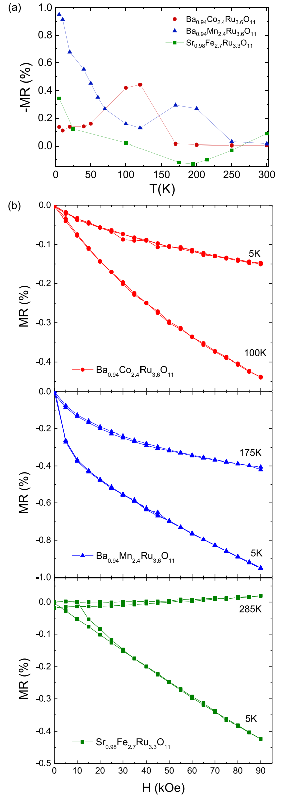
FIG. 10. (a) (-\text{MR}) of Co-, Mn-, and Fe-124 oxides as a function of temperature at 9 T with MR defined as 100 \times [(\rho(H) - \rho(0))/\rho(0)] , and MR as a function of magnetic field in (b).
