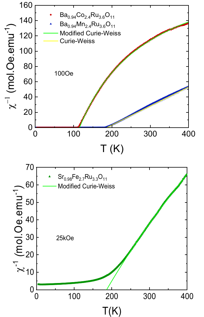
FIG. 6. Temperature-dependent inverse DC magnetic \chi^{-1}(T) in 100 Oe for \text{Ba}_{0.94}\text{Co}_{2.4}\text{Ru}_{3.6}\text{O}_{11} and \text{Ba}_{0.94}\text{Mn}_{2.4}\text{Ru}_{3.6}\text{O}_{11} (a) and in 25 kOe for \text{Sr}_{0.98}\text{Fe}_{2.7}\text{Ru}_{3.3}\text{O}_{11} (b), with the Curie-Weiss fitting (parameters are given in Table IV).
