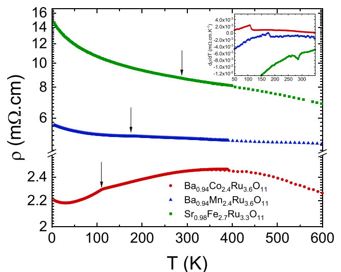
FIG. 8. Temperature-dependent resistivity. Arrows denotes the magnetic transitions. Inset: d\rho/dT curves.
