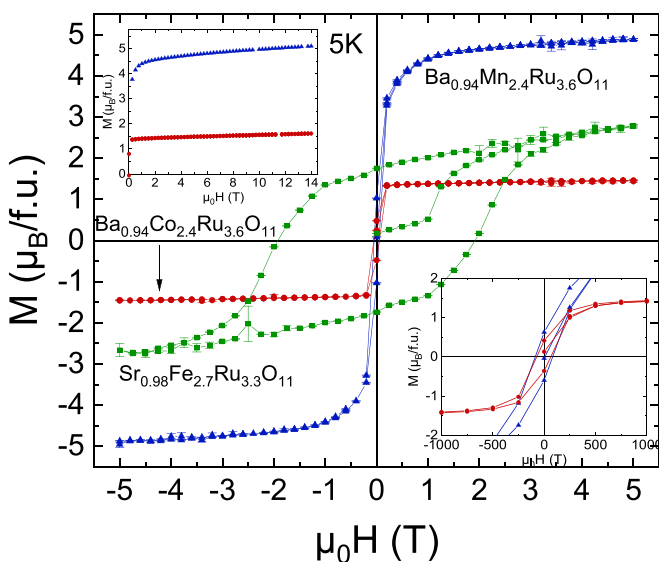
FIG. 7. Field-dependent magnetization at 5 K with, for Mn (blue), Co- (red), and Fe- (green) 124 oxides, low-field magnetization (lower inset) and high-field magnetization up to 14 T (upper inset).
