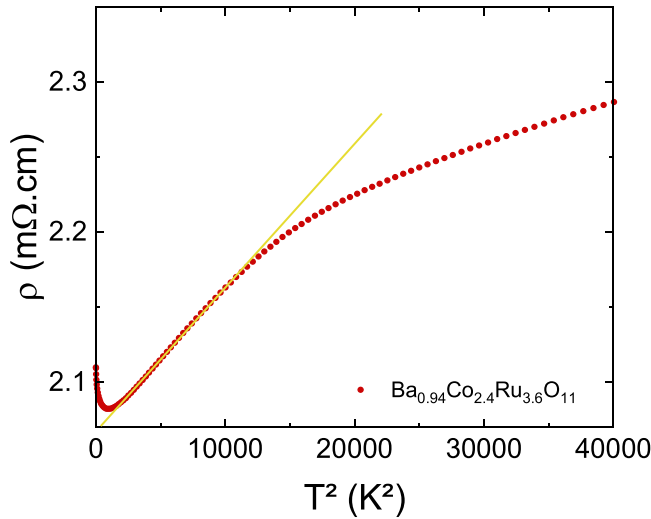
FIG. 9. T^2 -dependent resistivity of \text{Ba}_{0.94}\text{Co}_{2.4}\text{Ru}_{3.6}\text{O}_{11} . Also shown is the linear fit (yellow) to the data in the range 50 to 90 K.
