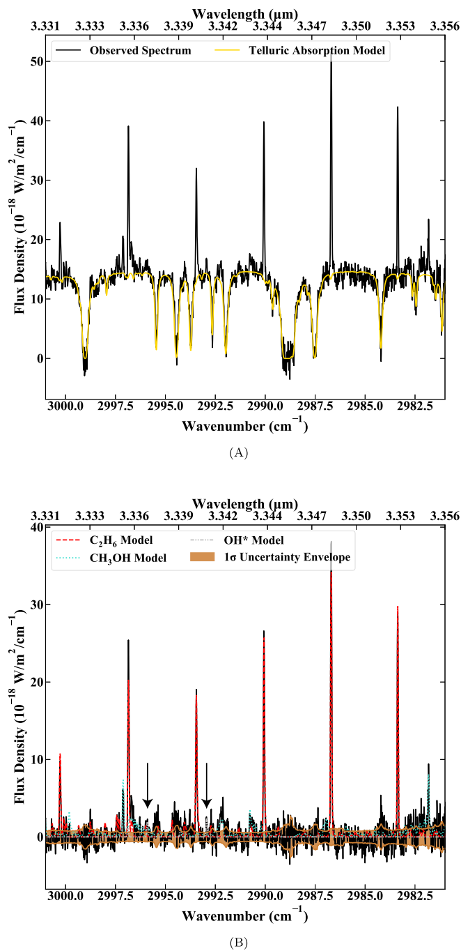
Figure 1. (A) Extracted iSHELL spectrum showing detections of \text{C}_2\text{H}_6 , \text{CH}_3\text{OH} , and \text{OH}^* in Wirtanen on UT 2018 December 18. The gold trace overplotted on the uppermost cometary spectrum is the telluric absorption model (convolved to the instrumental resolution and scaled to the observed continuum level). (B) Residual emission spectrum (after subtracting the telluric absorption model) with individual fluorescence models overlaid (color coded and styled by species) and the 1\sigma uncertainty envelope shaded in bronze. Arrows indicate positions of \text{OH}^* lines.
