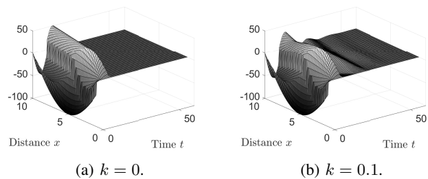
Fig. 3: Second observer on [\delta, L] (boundary observer).
