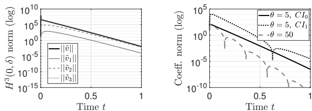
(a) State error for \theta = 5 .
