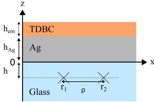
FIG. 1. Layout of the photoluminescence system. The structure consists in a layer of TDDBC on top of a 45-nm-thick layer ( h_{\text{Ag}} ) of silver. These layers are deposited on a glass substrate. The cross-spectral density tensor is calculated at the points \mathbf{r}_1 and \mathbf{r}_2 , separated by the distance \rho = |\mathbf{r}_2 - \mathbf{r}_1| at a distance h = 1 \mu\text{m} from the silver layer. The TDDBC layer ( h_{\text{em}} ) is either 5-nm or 20-nm-thick.
