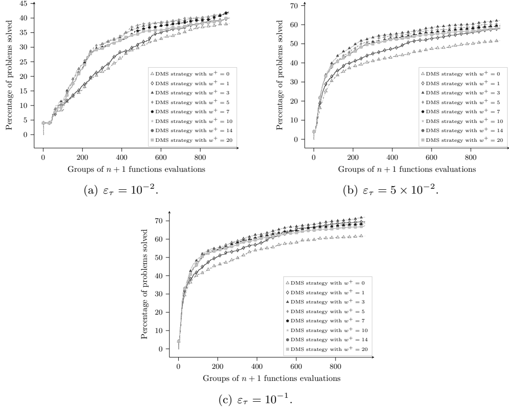
Figure 16: Data profiles obtained on 10 replications from 100 multiobjective optimization problems from [22] for DMulti-MADS variants with DMS strategy with tolerance \varepsilon_\tau \in \{10^{-2}, 5 \times 10^{-2}, 10^{-1}\} .
