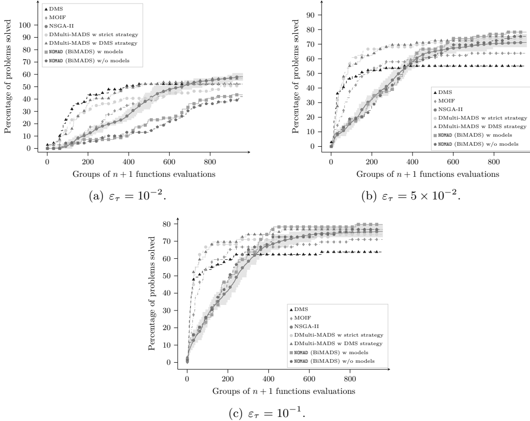
Figure 14: Data profiles using NOMAD (BiMADS), DMS, DMulti-MADS, MOIF and NSGA-II obtained on 69 biobjective optimization problems from [22] with 50 different runs of NSGA-II with tolerance \varepsilon_\tau \in \{10^{-2}, 5 \times 10^{-2}, 10^{-1}\} .
