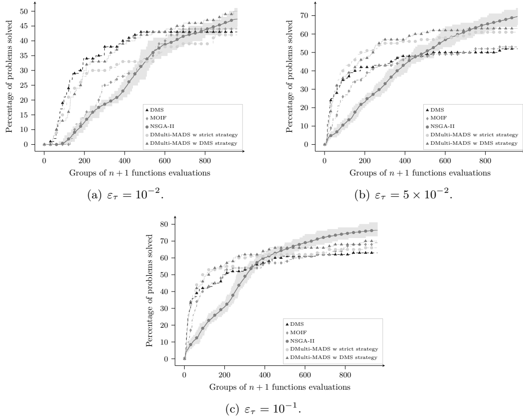
Figure 13: Data profiles using DMS, DMulti-MADS, MOIF and NSGA-II obtained on 100 multiobjective optimization problems (69 with m = 2 , 29 with m = 3 and 2 with m = 4 ) from [22] with 50 different runs of NSGA-II with tolerance \varepsilon_\tau \in \{10^{-2}, 5 \times 10^{-2}, 10^{-1}\} .
