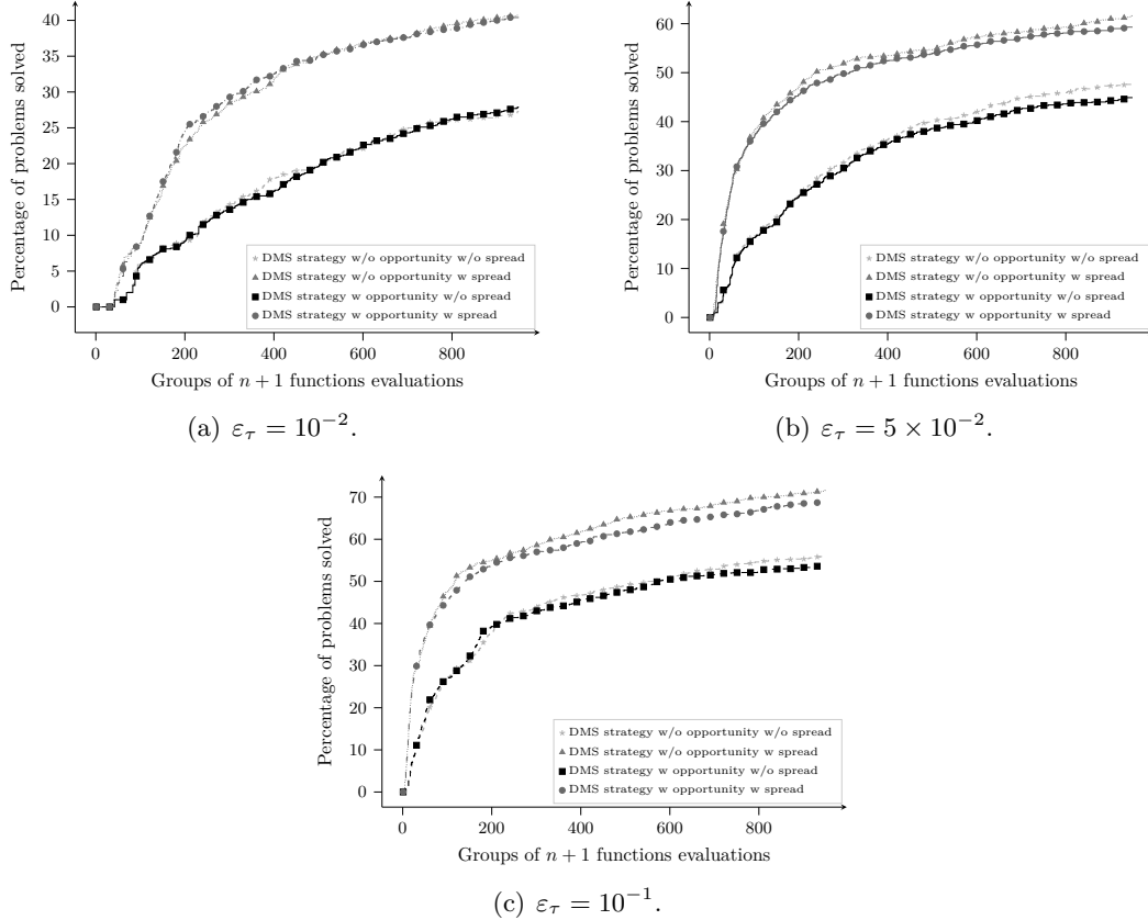
Figure 11: Data profiles obtained on 10 replications from 100 multiobjective optimization problems from [22] for DMulti-MADS variants with DMS strategy with tolerance \varepsilon_\tau \in \{10^{-2}, 5 \times 10^{-2}, 10^{-1}\} .
