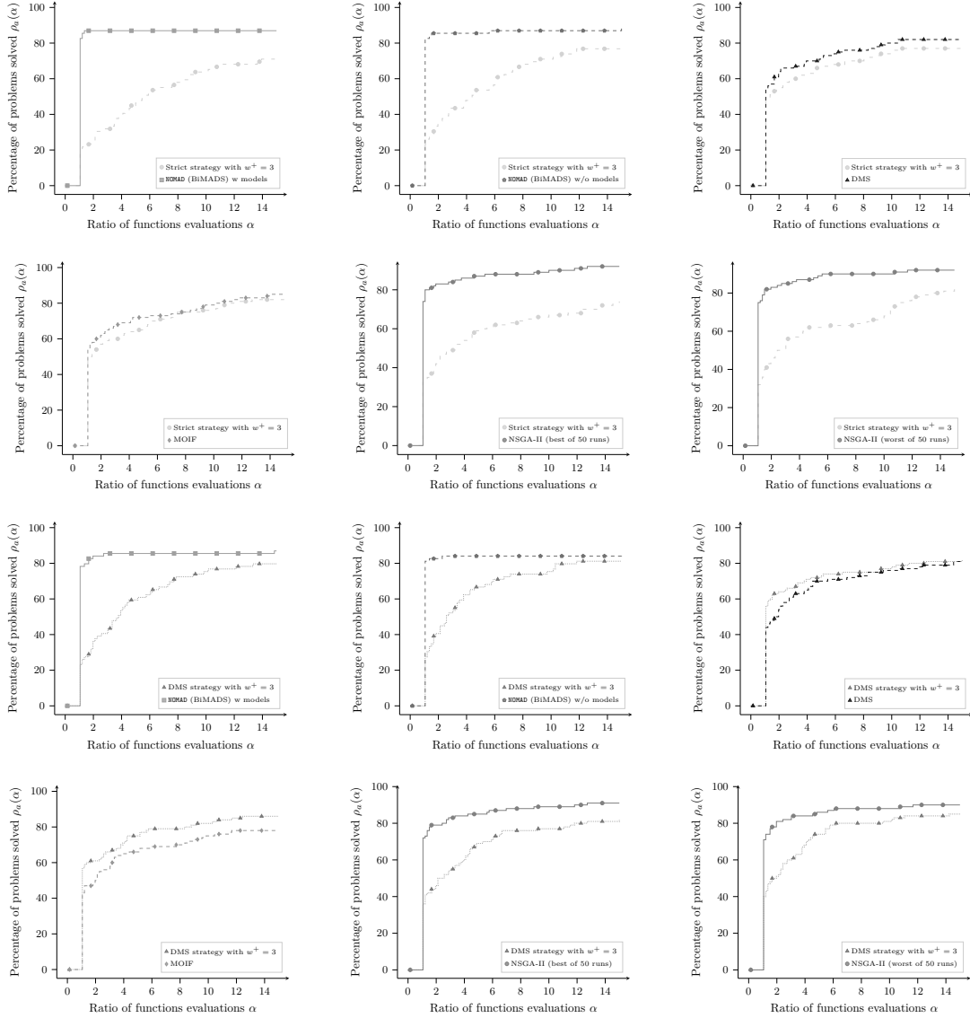
Figure 19: \Gamma spread performance profiles using NOMAD (BiMADS), DMS, DMulti-MADS with DMS strategy, MOIF and NSGA-II obtained on 100 multiobjective optimization problems (69 with m = 2 , 29 with m = 3 and 2 with m = 4 ) from [22] with 50 different runs of NSGA-II.
