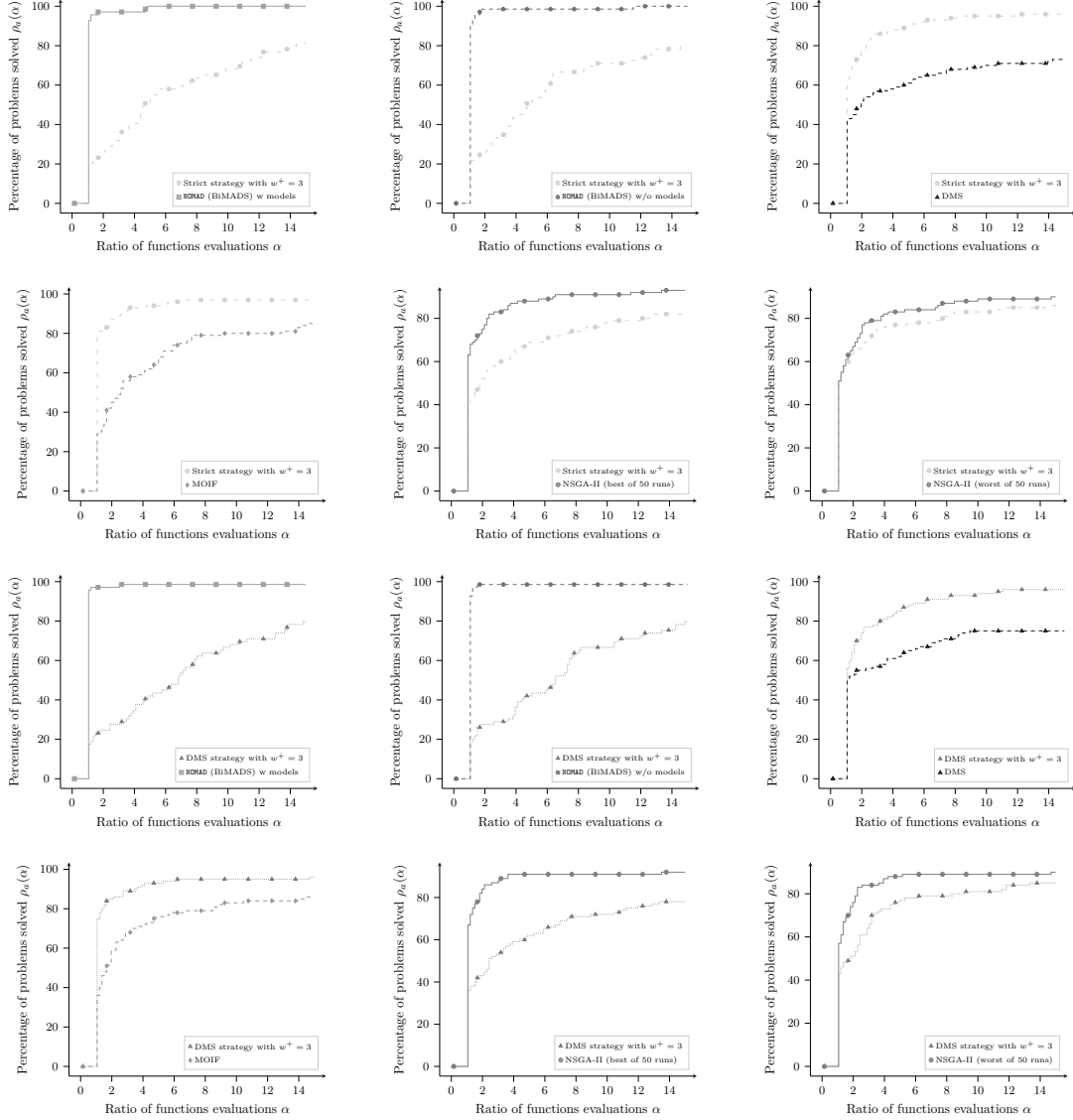
Figure 17: Purity performance profiles using NOMAD (BiMADS), DMS, DMulti-MADS, MOIF and NSGA-II obtained on 100 multiobjective optimization problems (69 with m = 2 , 29 with m = 3 and 2 with m = 4 ) from [22] with 50 different runs of NSGA-II.
