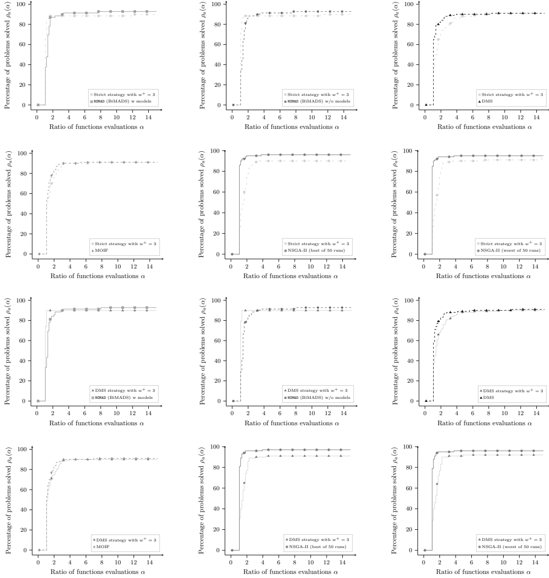
Figure 18: \Delta spread performance profiles using NOMAD (BiMADS), DMS, DMulti-MADS, MOIF and NSGA-II obtained on 100 multiobjective optimization problems (69 with m = 2 , 29 with m = 3 and 2 with m = 4 ) from [22] with 50 different runs of NSGA-II.
