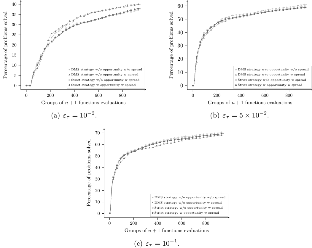
Figure 12: Data profiles obtained on 10 replications from 100 multiobjective optimization problems from [22] for the four best DMulti-MADS variants with tolerance \varepsilon_\tau \in \{10^{-2}, 5 \times 10^{-2}, 10^{-1}\} .
