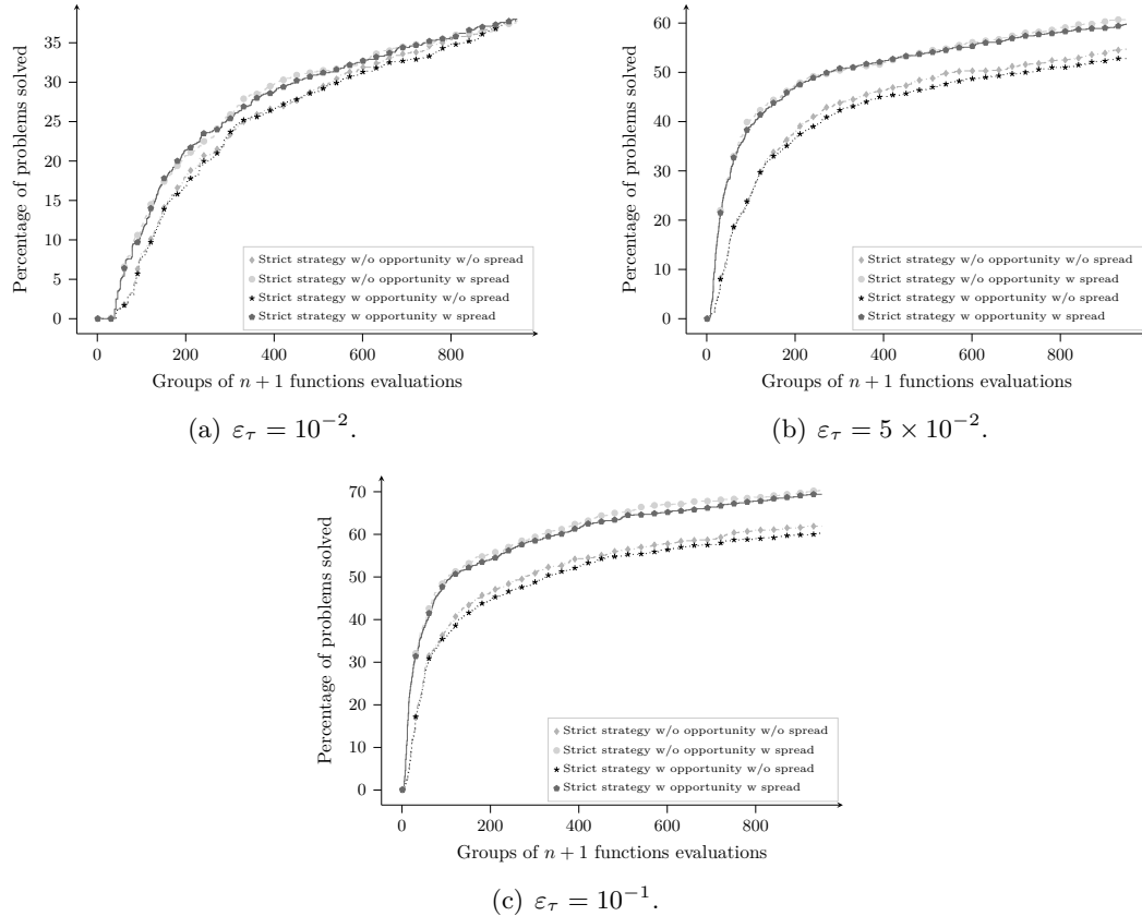
Figure 10: Data profiles obtained on 10 replications from 100 multiobjective optimization problems from [22] for DMulti-MADS strict success strategy variants with tolerance \varepsilon_\tau \in \{10^{-2}, 5 \times 10^{-2}, 10^{-1}\} .
