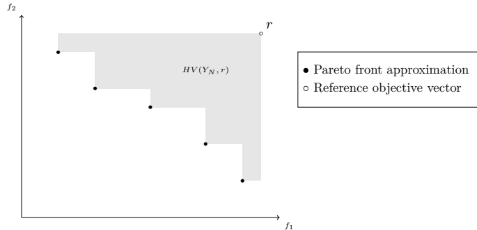
Figure 9: Illustration of the hypervolume indicator (HV) for a biobjective minimization problem, delimited above by the reference objective vector r \in \mathbb{R}^2 . The higher, the better.
