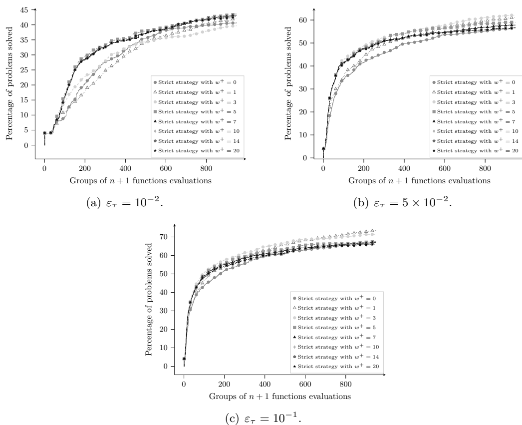
Figure 15: Data profiles obtained on 10 replications from 100 multiobjective optimization problems from [22] for DMulti-MADS variants with strict success strategy without opportunistic polling and with spread strategy for tolerance \varepsilon_\tau \in \{10^{-2}, 5 \times 10^{-2}, 10^{-1}\} .
