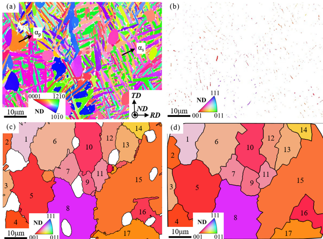
Fig. 3. IPF maps of Sample A, (a) \alpha phase and (b) \beta phase. \alpha_p is globular primary \alpha grain and \alpha_s represents secondary \alpha colony. (c) and (d) are IPF maps of parent \beta grains reconstructed by misorientation criterion and denoising method, respectively. The numbers of 17 grains in (c) and equivalent grains in (d) are labeled.
