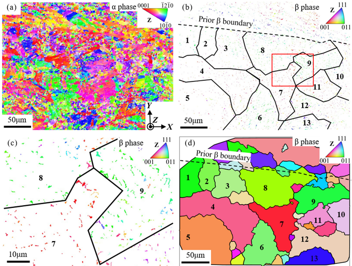
Fig. 6. IPF map of Sample B, (a) \alpha phase and (b) \beta phase. (c) The higher-magnification IPF map of the area in the red box of (b). (d) IPF map of parent \beta grains reconstructed from (b) by denoising method. The \beta grain boundaries are marked by black lines. The numbers of 13 grains in (b) and equivalent grains in (d) are labeled. (For interpretation of the references to color in this figure legend, the reader is referred to the web version of this article.)
