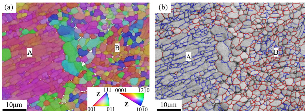
Fig. 11. EBSD maps of the heterogeneous area of Sample B, (a) Band contrast image overlaid with an IPF map colored by the shown color bars. (b) Band contrast map with colored grain boundaries. The red and blue lines represent HAGBs and LAGBs, respectively. (For interpretation of the references to color in this figure legend, the reader is referred to the web version of this article.)
