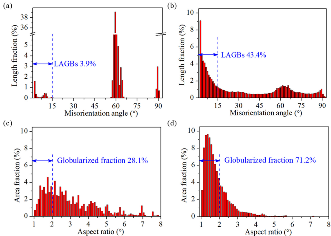
Fig. 10. Distributions of (a) \alpha - \alpha boundary misorientation angle of initial Sample B, (b) \alpha - \alpha boundary misorientation angle of deformed Sample B, (c) grain shape aspect ratio of initial Sample B and (d) grain shape aspect ratio of deformed Sample B.
