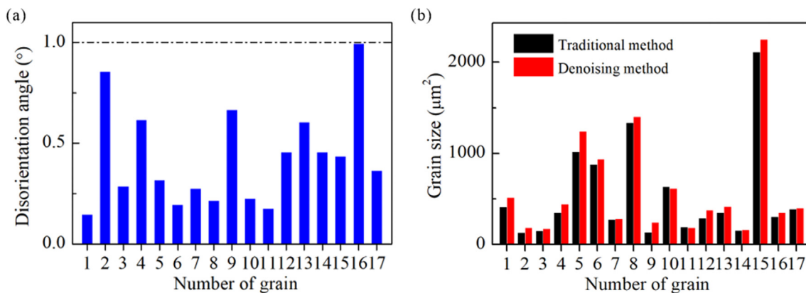
Fig. 4. Distributions of (a) disorientation angle and (b) grain size. The orientations and sizes of the 17 grain are calculated by traditional and denoising reconstruction method.
