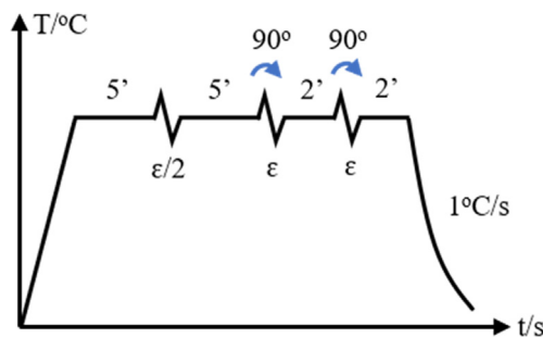
Fig. 2. Thermomechanical cycle on MaxStrain device ( \varepsilon = 40\% , \dot{\varepsilon} = 0.1 \text{ s}^{-1} ).
