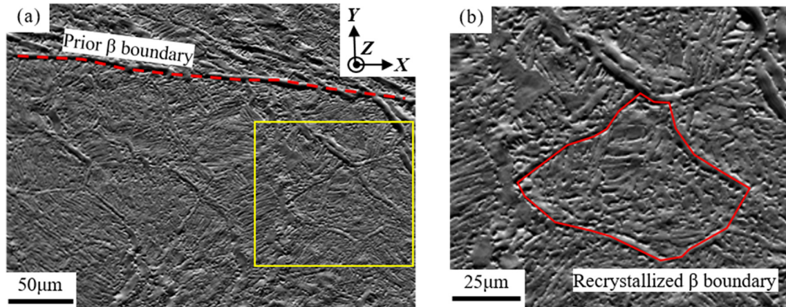
Fig. 5. (a) FSD image of Sample B. (b) The higher-magnification FSD image of the area in the yellow box. (For interpretation of the references to color in this figure legend, the reader is referred to the web version of this article.)
